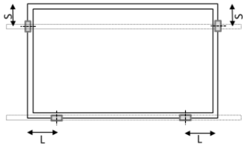
Fig. A3b: Clamp position on long & short frames Mounting rails parallel to the longer frame
