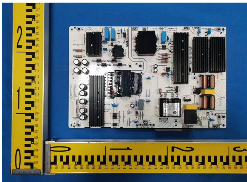
Figure 3. Power board
