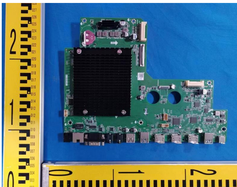
Figure 4. Mainboard view
