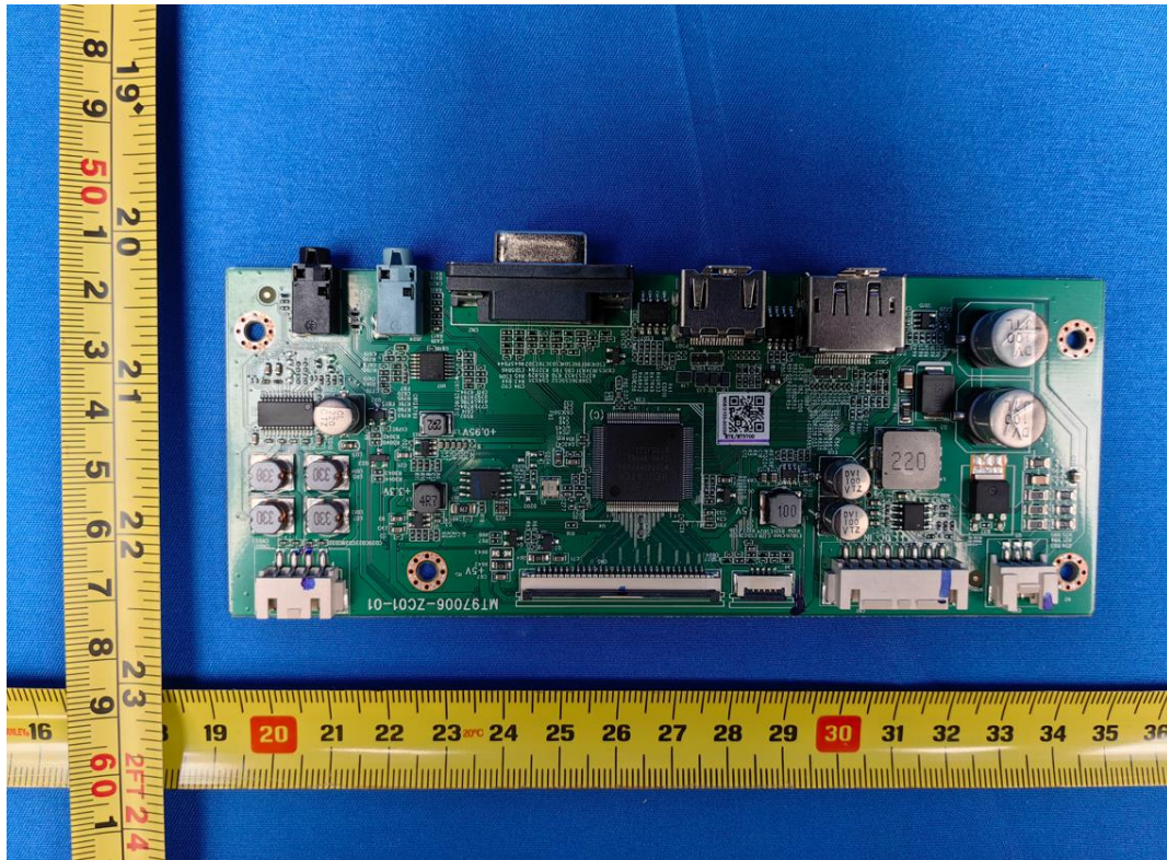
Figure 15 Component side of main board
