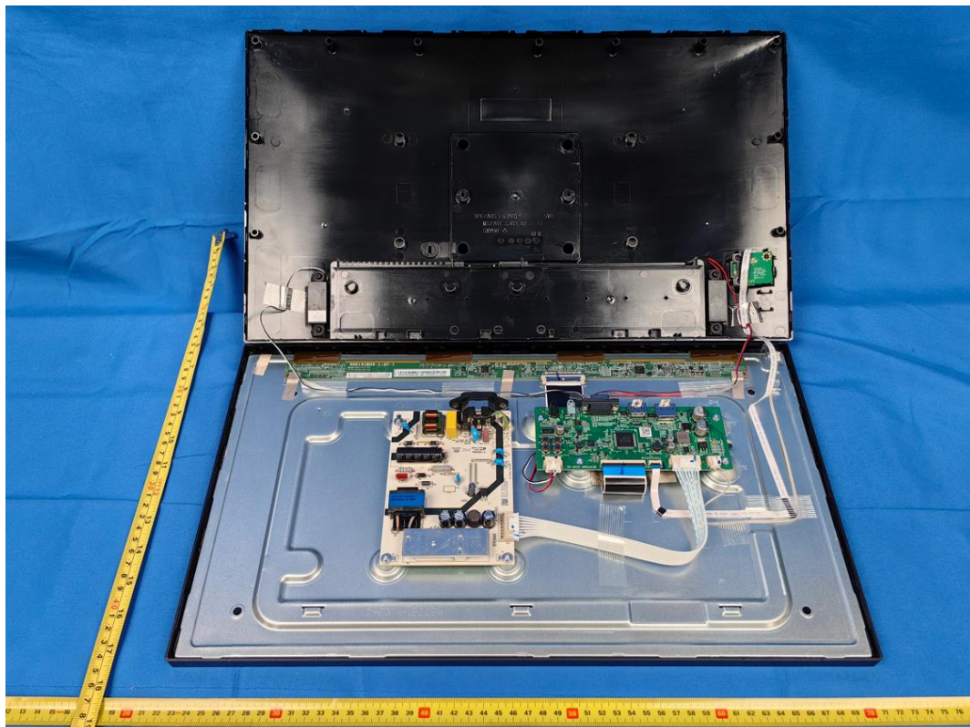
Figure 10 Internal view
