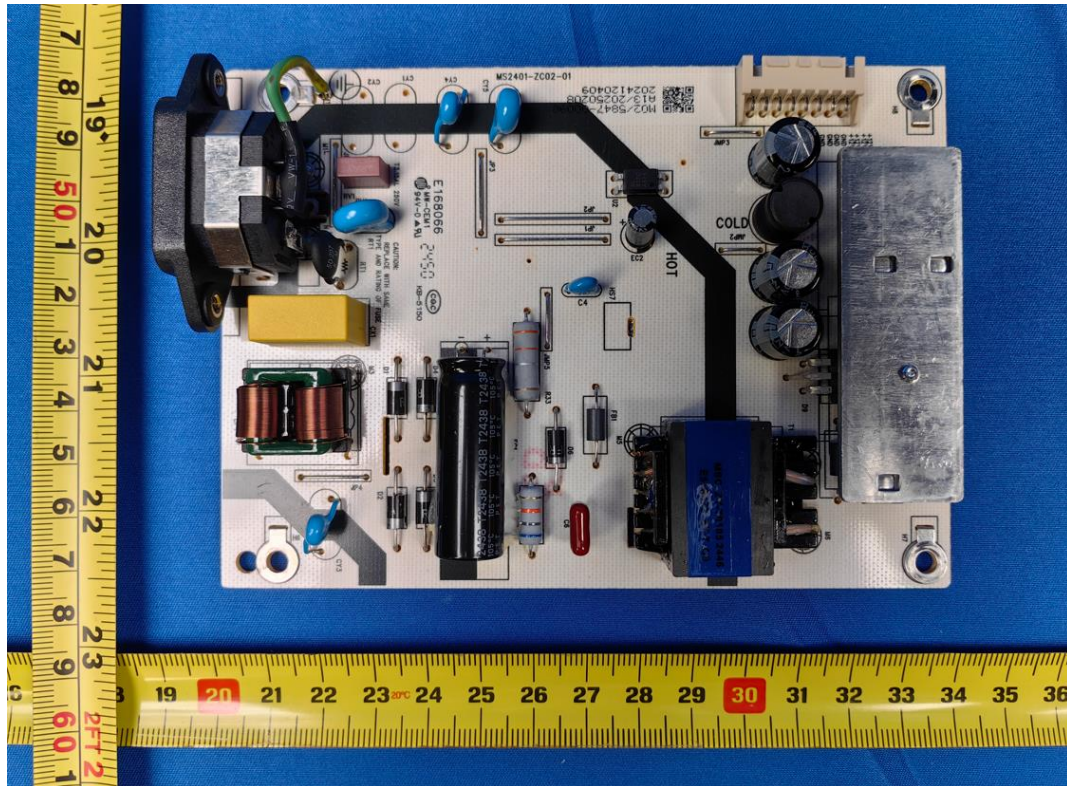
Figure 13 Component side of power board
