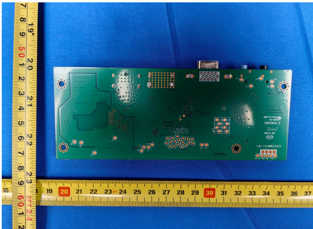
Figure 16 Trace side of main board
