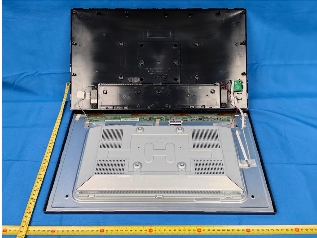
Figure 9 Internal view
