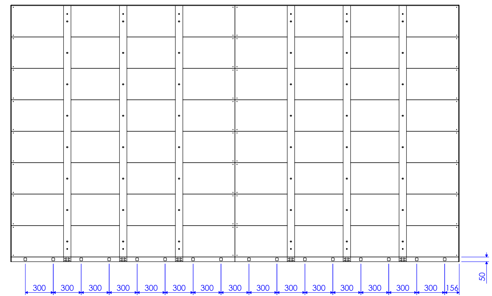
REAR VIEW CABLE HOLES
