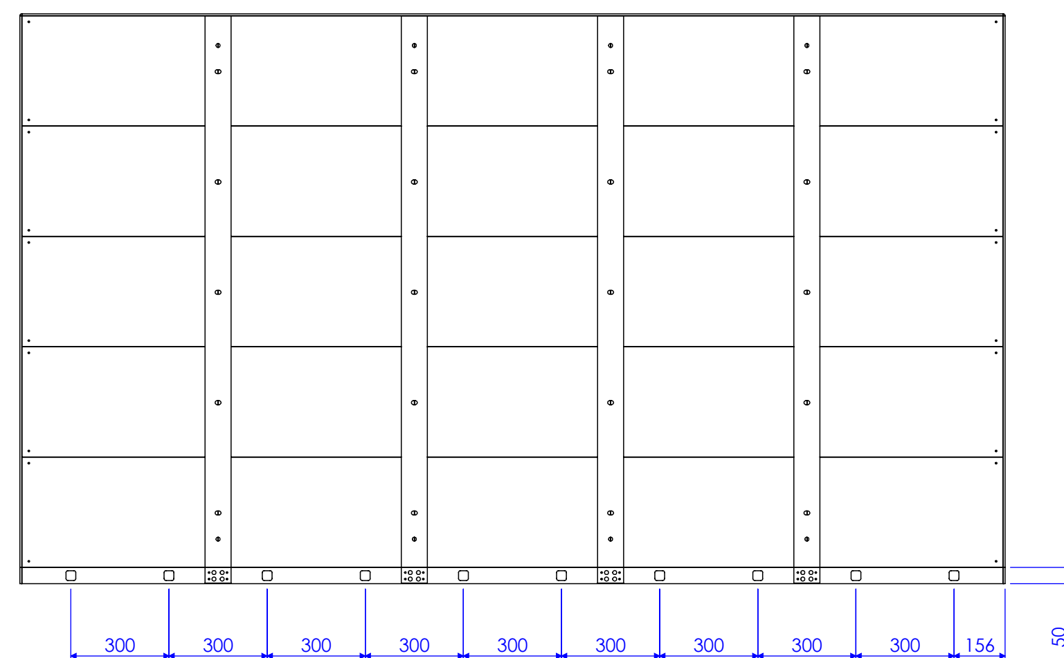
REAR VIEW CABLE HOLES
