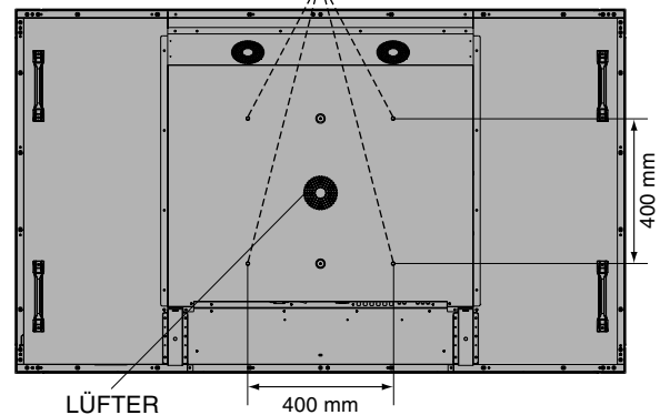
VESA-Montageadapter
