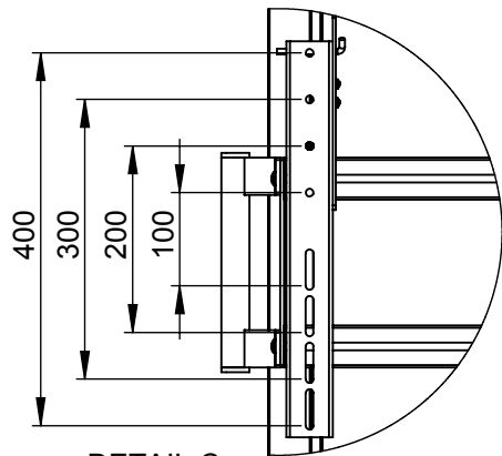
DETAIL C SCALE 1 : 9
