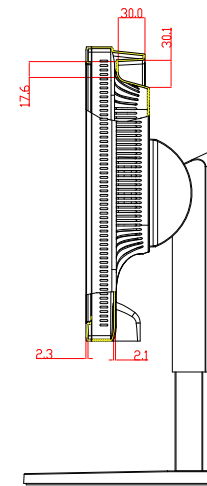
SECTION H-H
