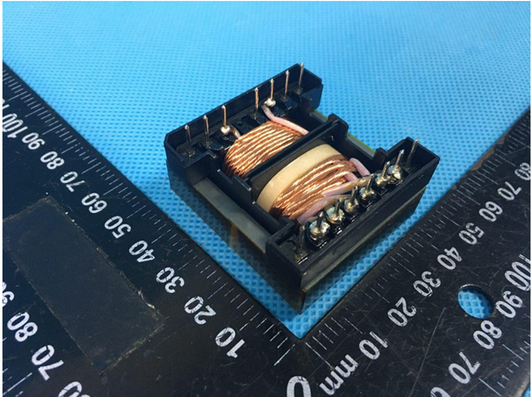
Photo 23 Transformer THA1 view
