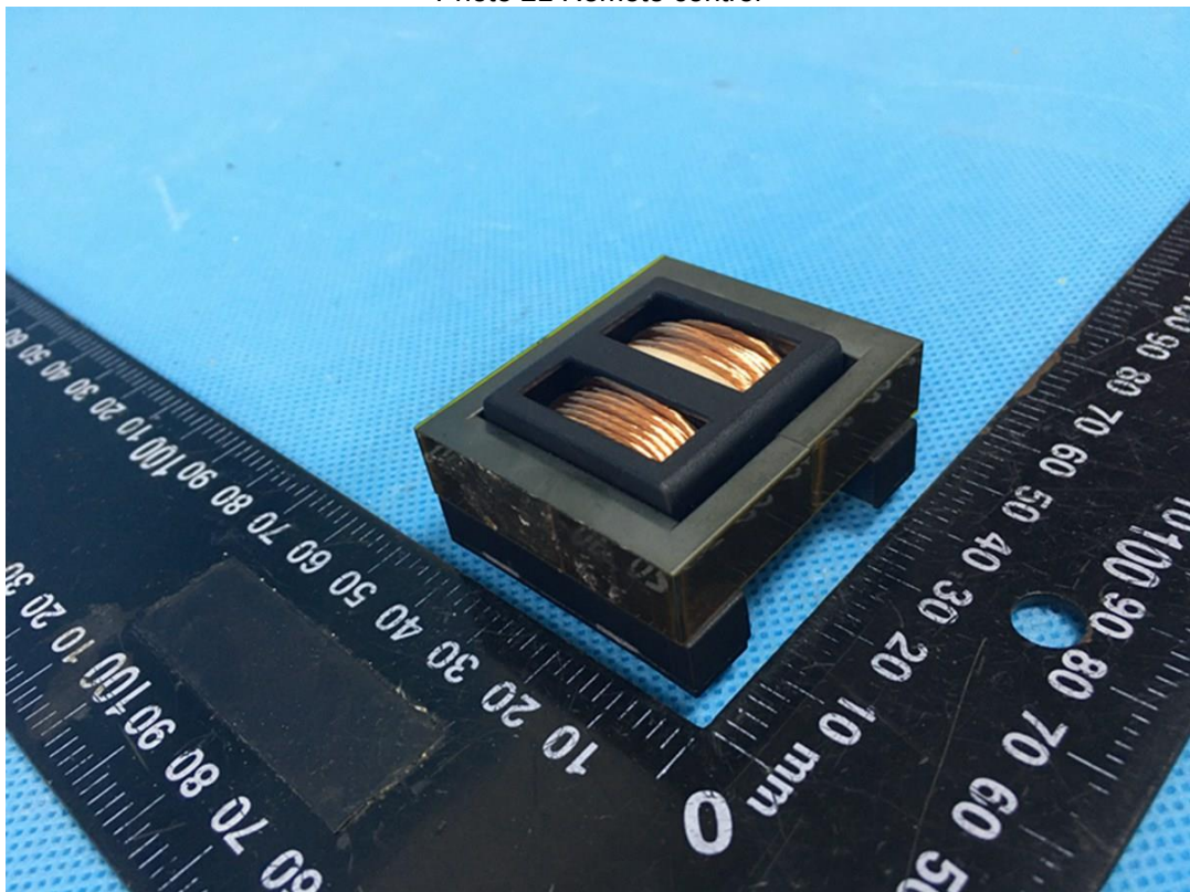
Photo 22 Transformer THA1 view
