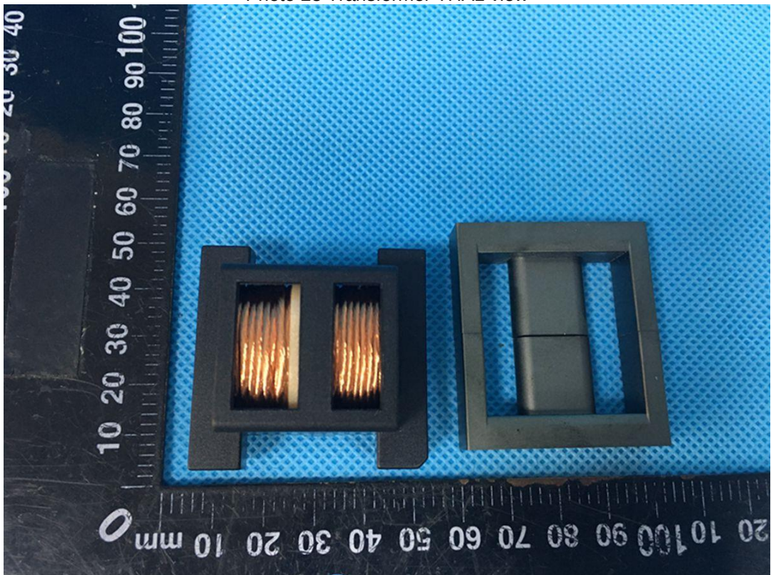
Photo 24 Transformer THA1 view
