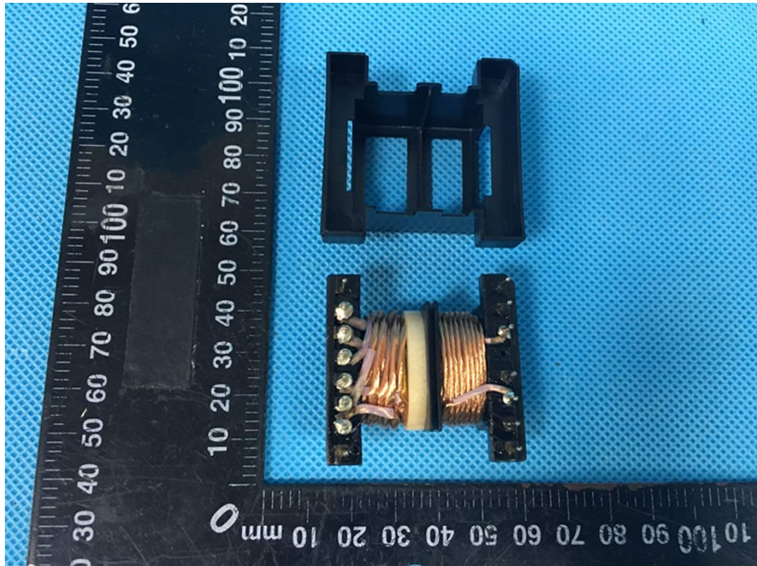
Photo 25 Transformer THA1 view
