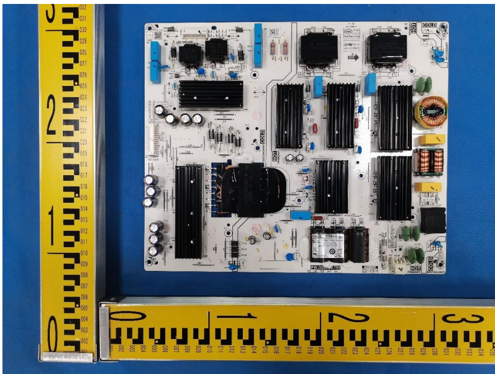
Figure 3. Power board
