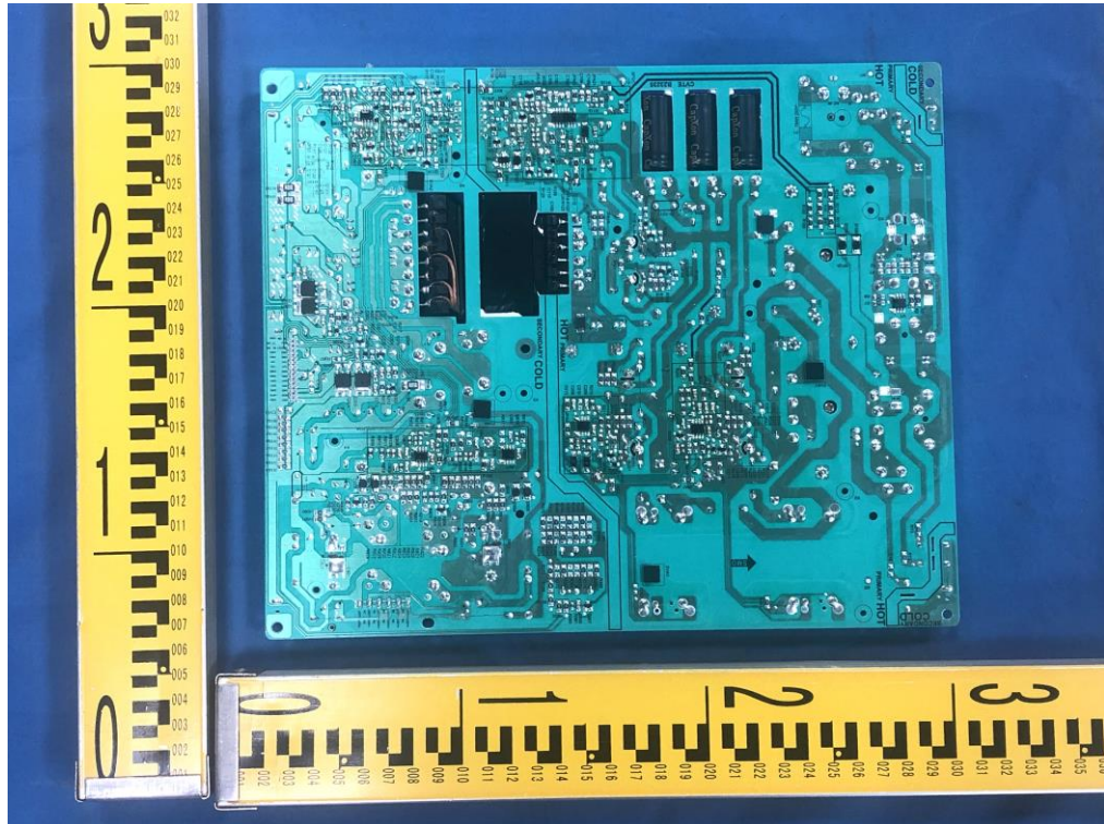
Figure 13 Switching Power Supply view
