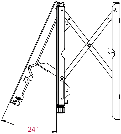
COMPONENT ACCESS
