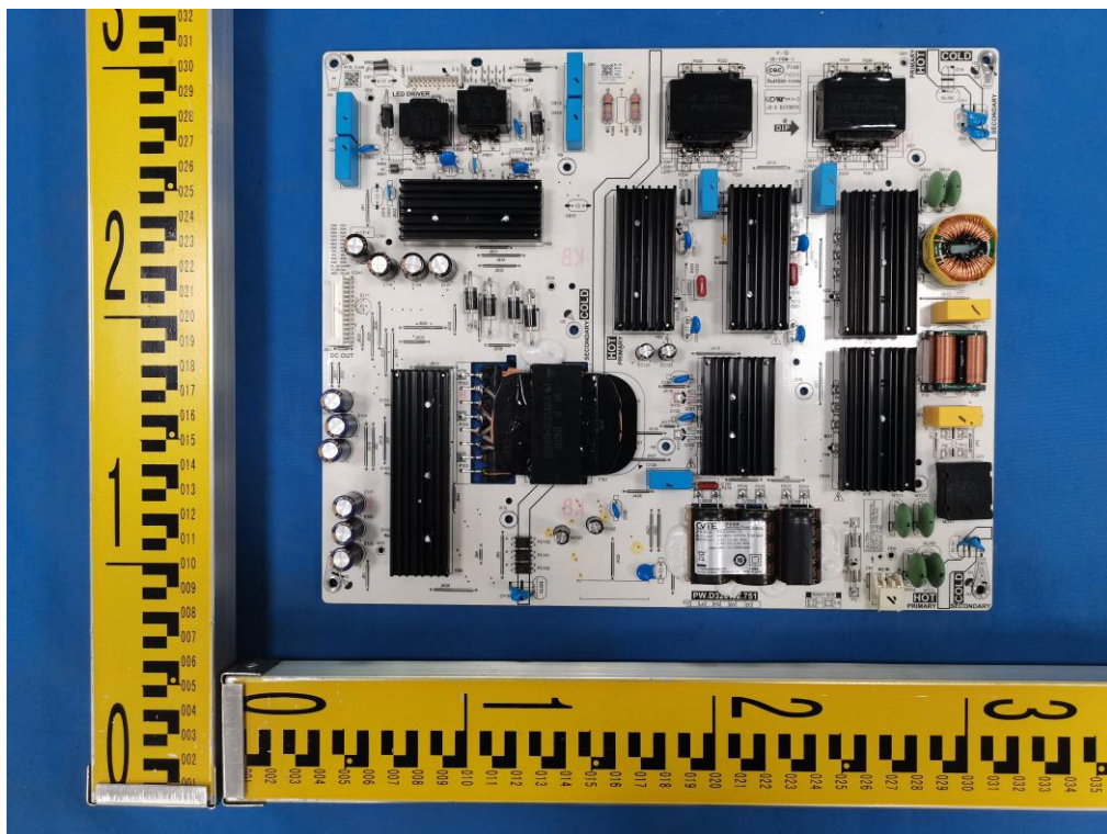
Figure 10. Switching Power Supply view
