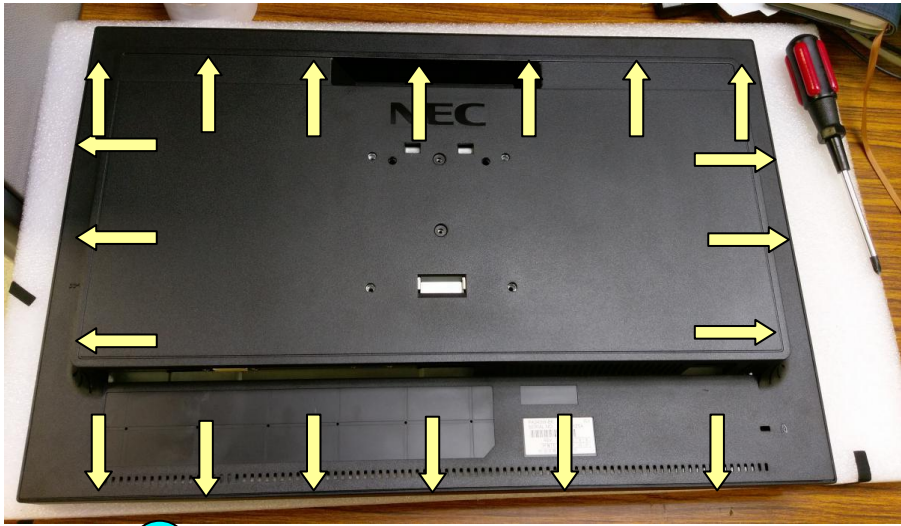
3 Disassemble the back cover
