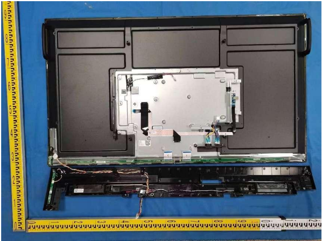
Figure 10. Internal view_3
