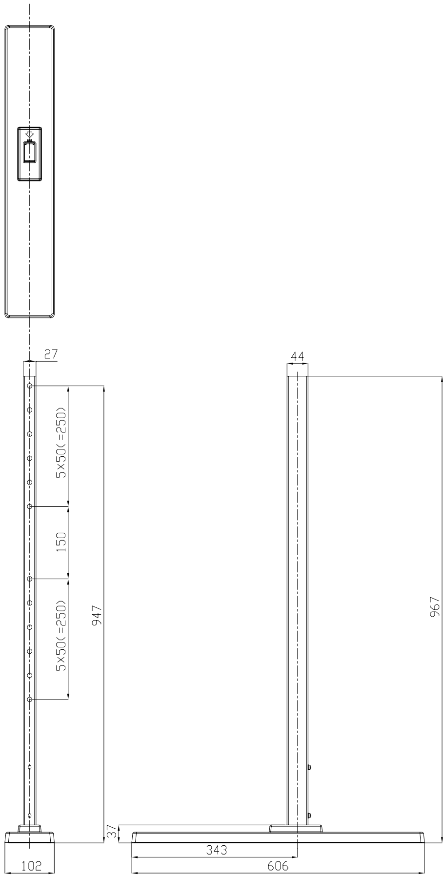
WITH PIPE
