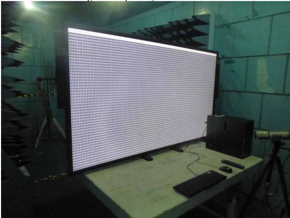
16.6. Photo of RF Strength Susceptibility Test
