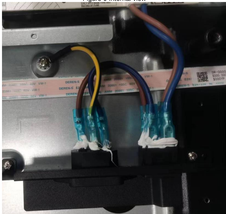
Figure 10 Internal view
