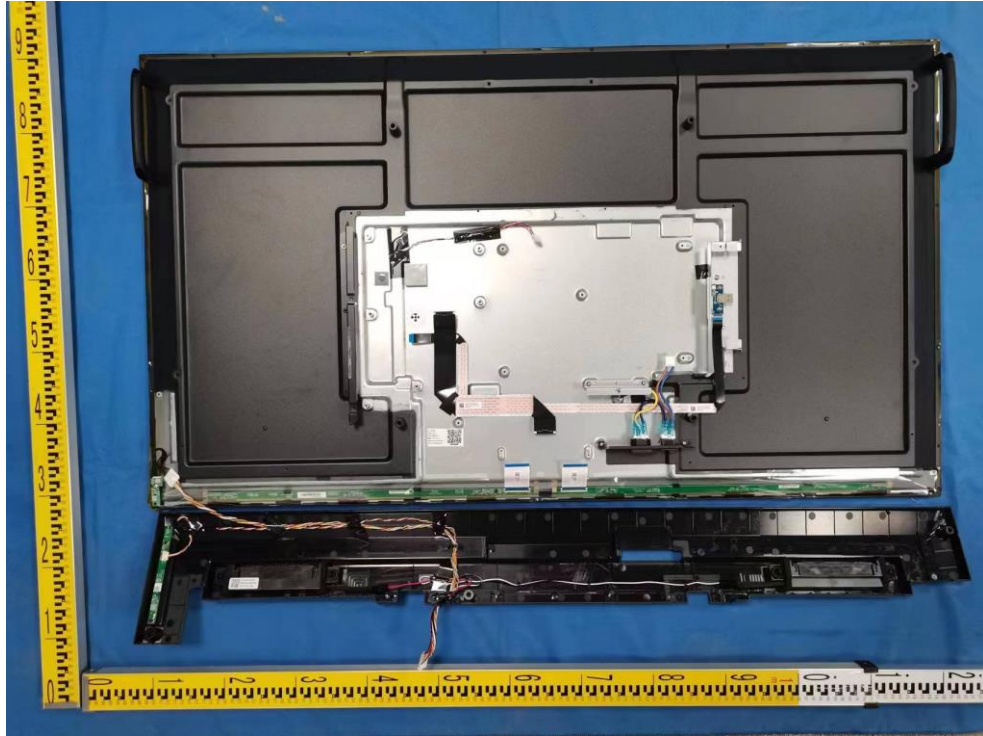
Figure 9 Internal view
