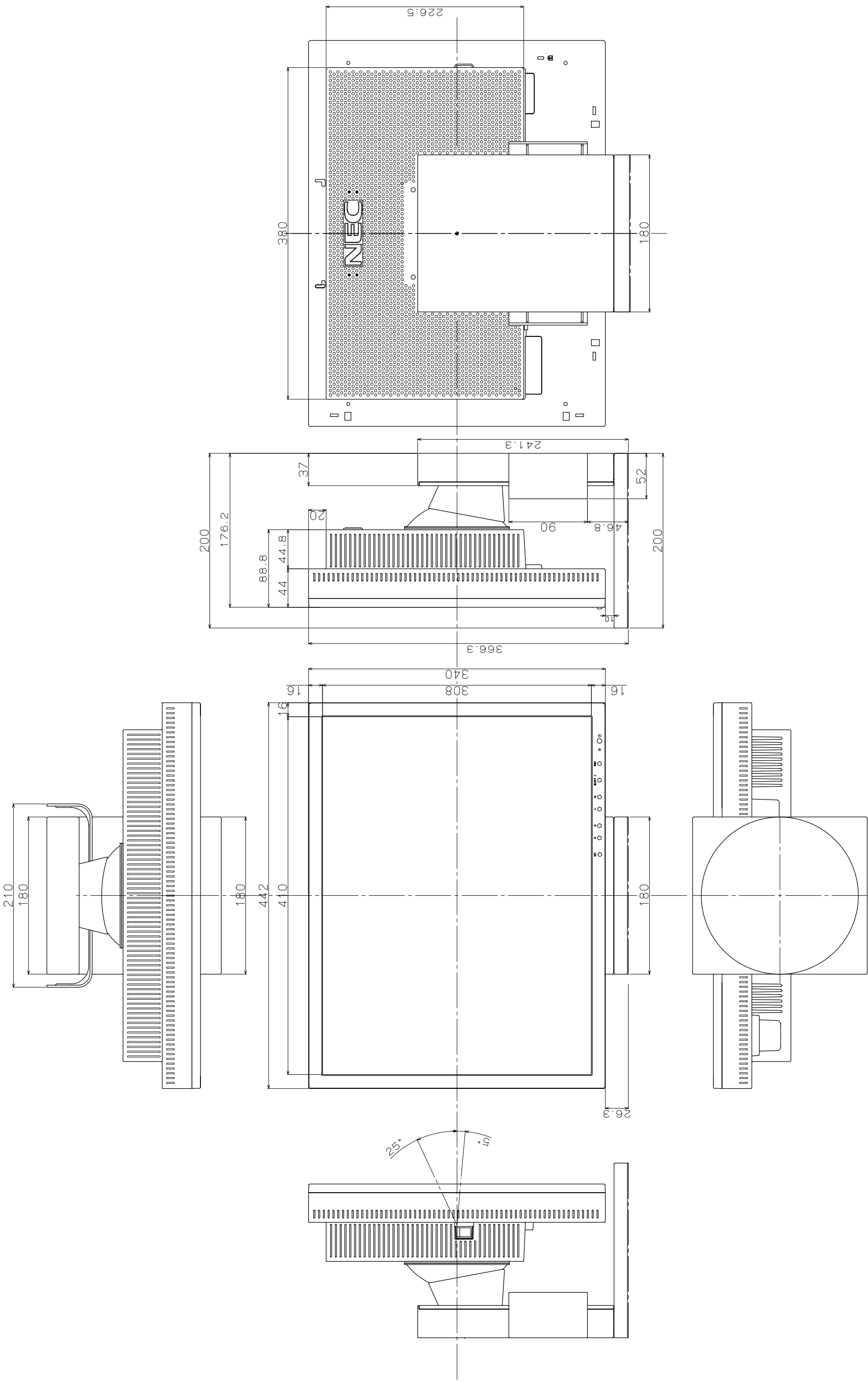
LCD2080UX Outside drawing
