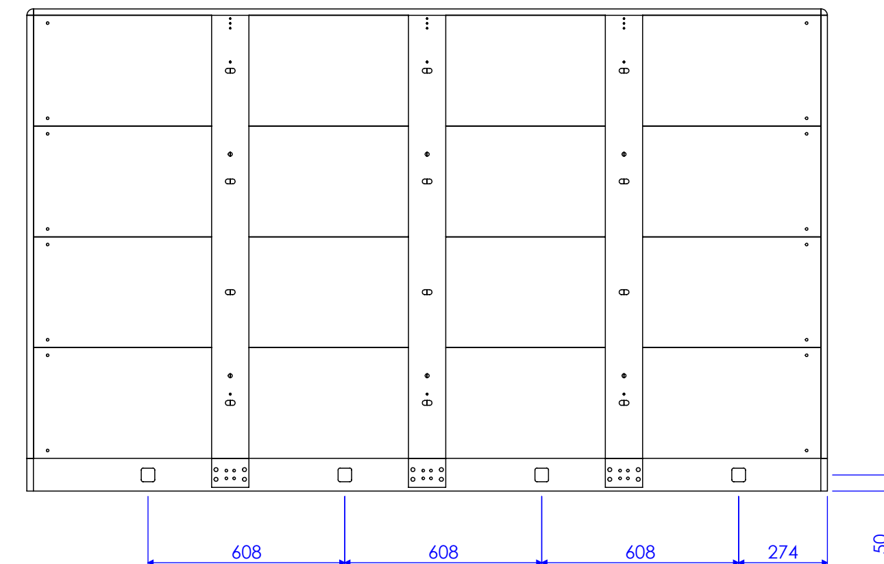
REAR VIEW CABLE HOLES
