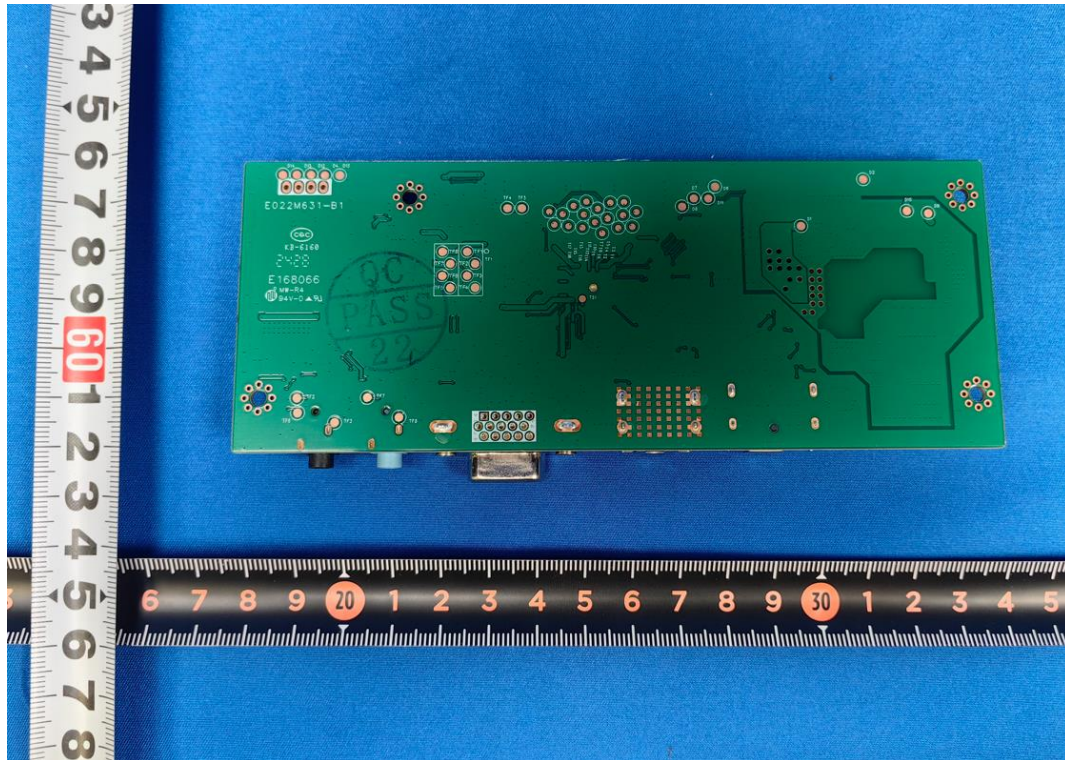
Figure 17 Trace side of main board
