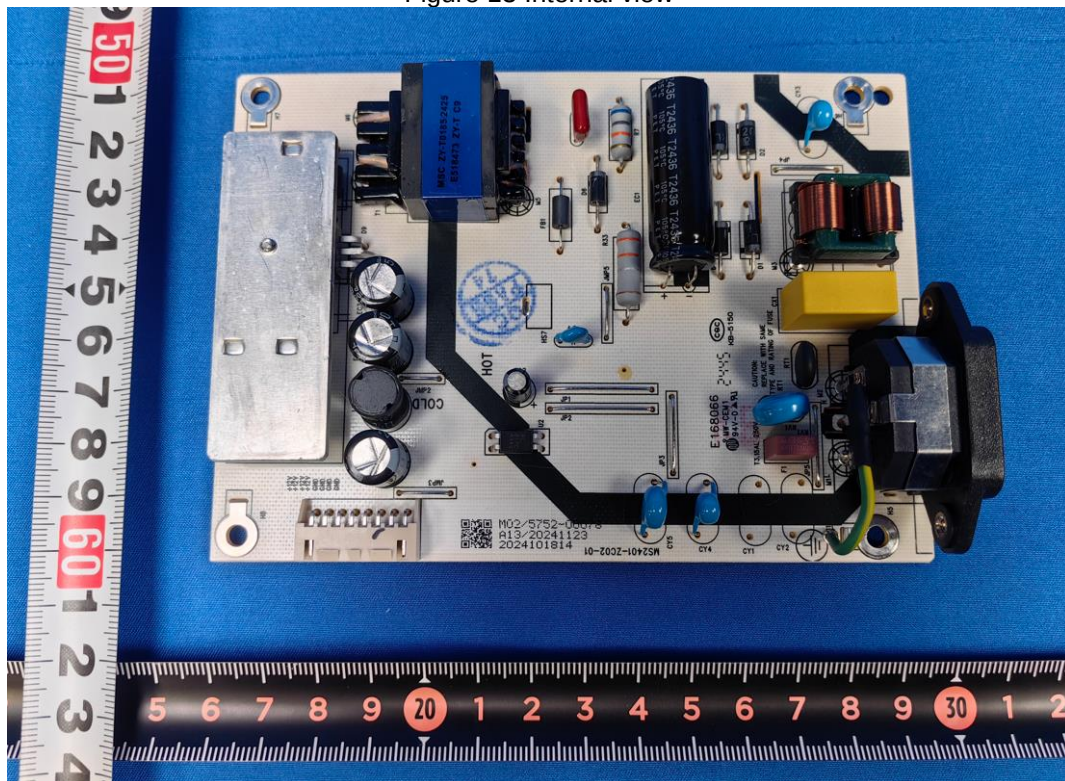
Figure 14 Component side of power board
