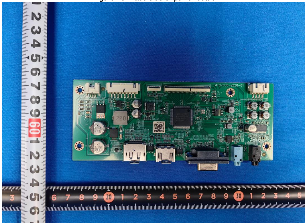
Figure 16 Component side of main board
