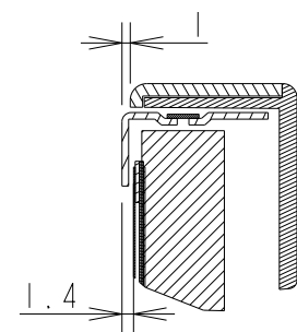
Section E-E Scale 1/1
