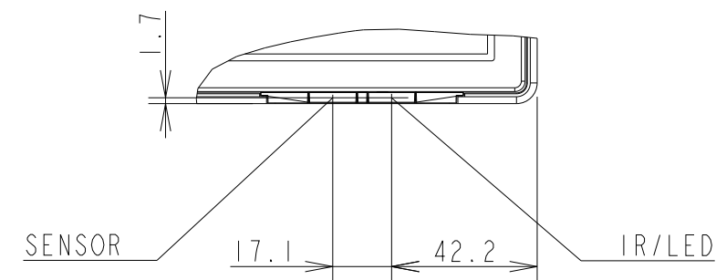
DETAIL B SCALE 1/2
