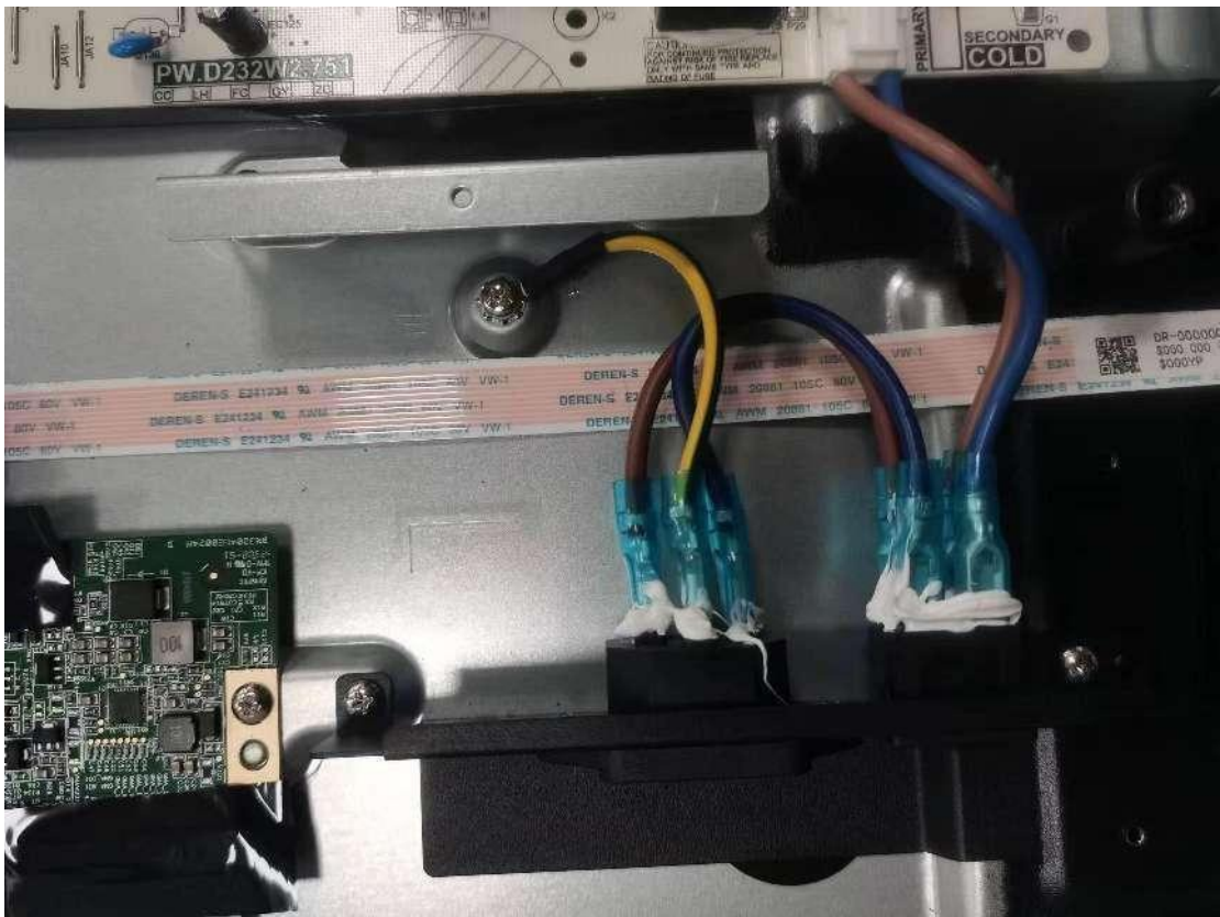
Figure 17. Bonding terminal view
