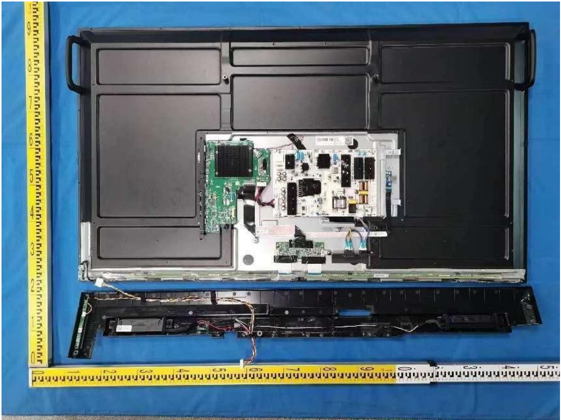
Figure 9. Internal view_2
