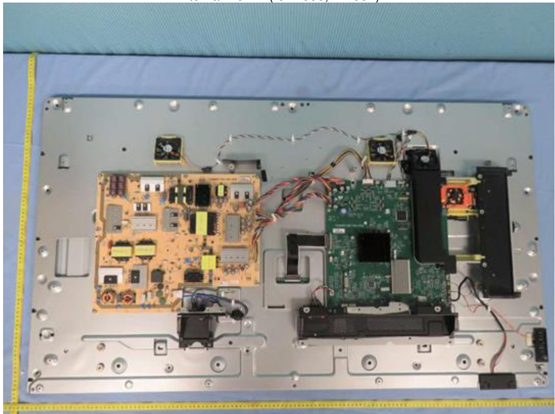
Internal view 1 (for P555, MA551)
