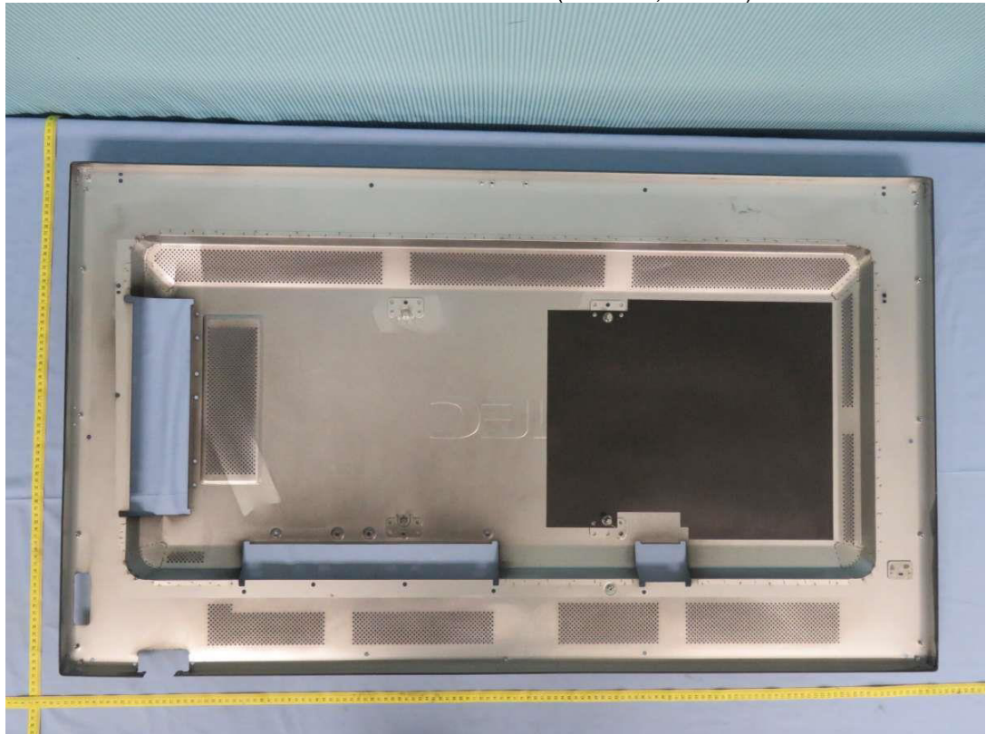
Metal enclosure internal view (for P555, MA551)
