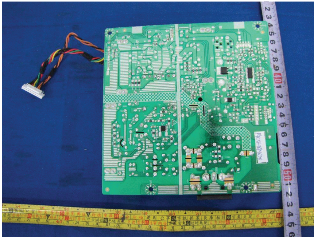
Figure 11. Power board 715G3727
