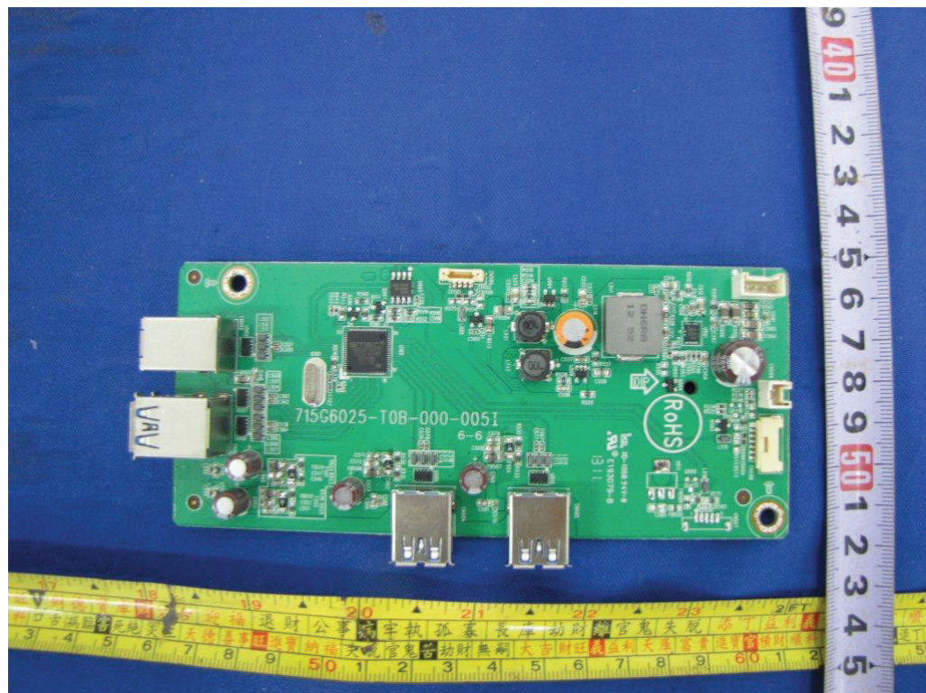
Figure 14. USB board 715G6025
