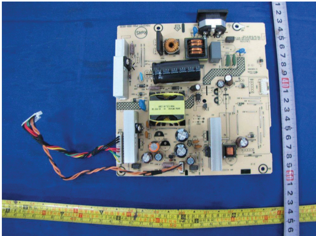
Figure 10. Power board 715G3727
