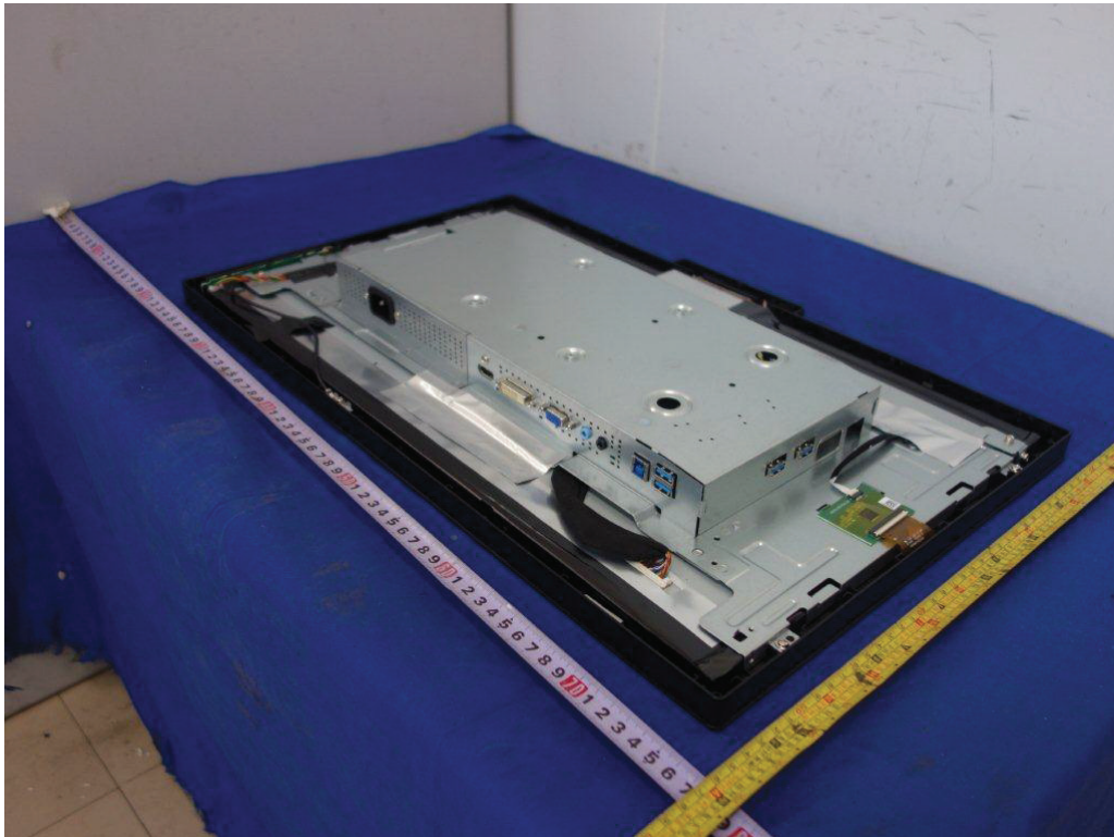
Figure 7. Metal enclosure
