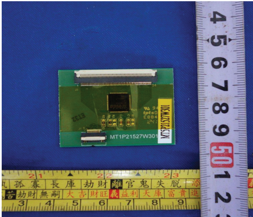
Figure 17. Touch-sensitive screen interfacing board MT1P21527W301
