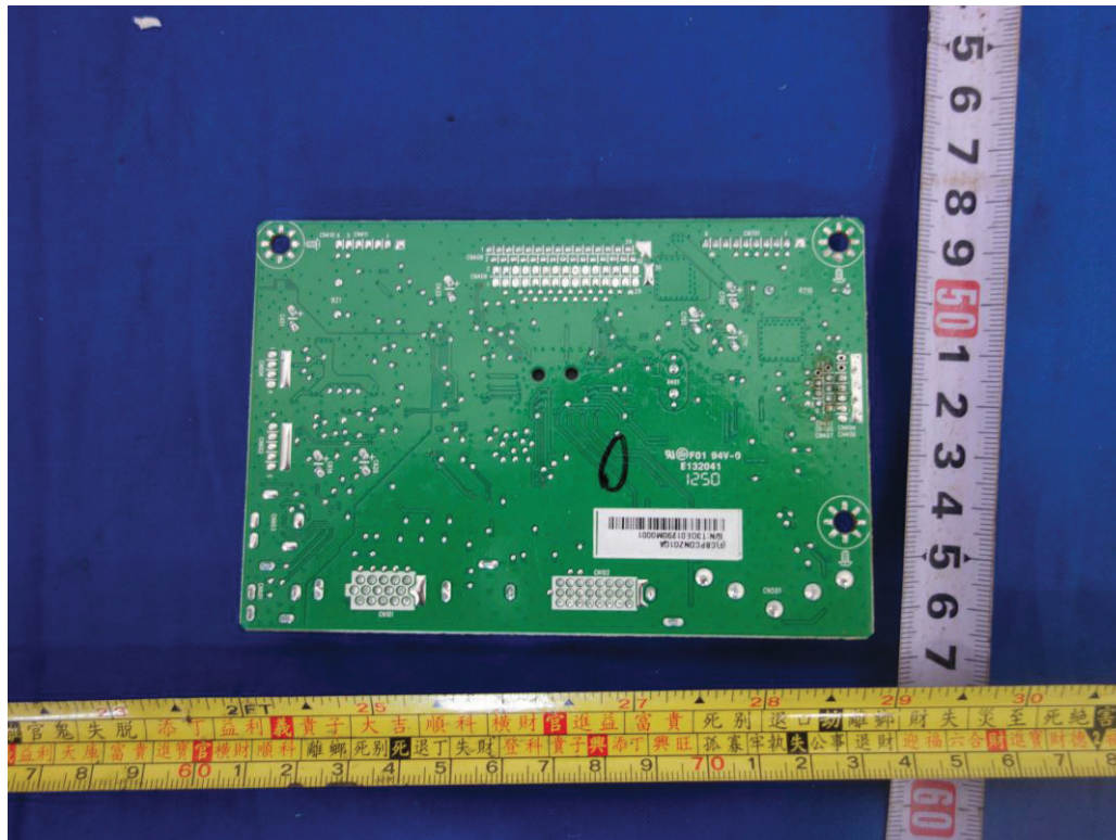
Figure 13. Main board 715G6654
