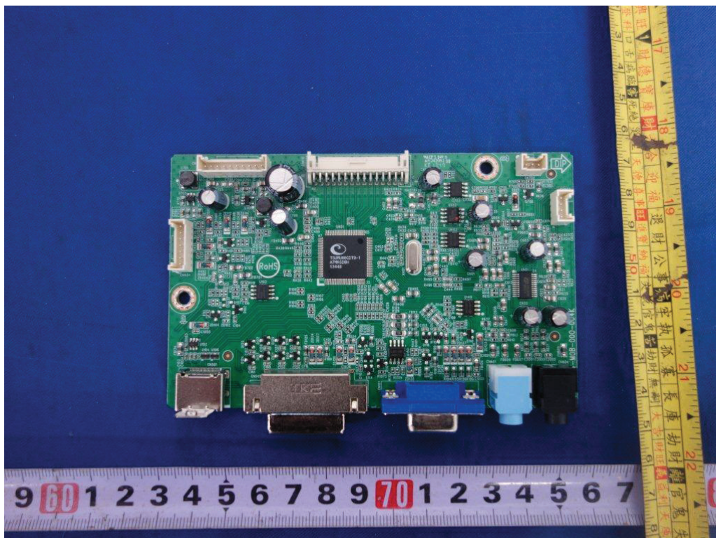
Figure 12. Main board 715G6654
