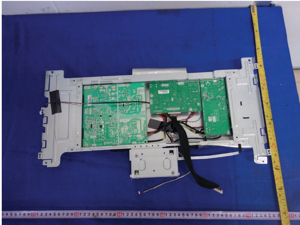
Figure 9. Internal view for metal enclosure
