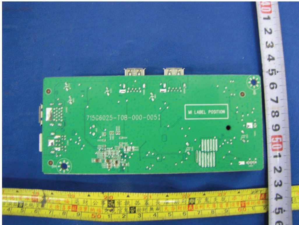
Figure 15. USB board 715G6025
