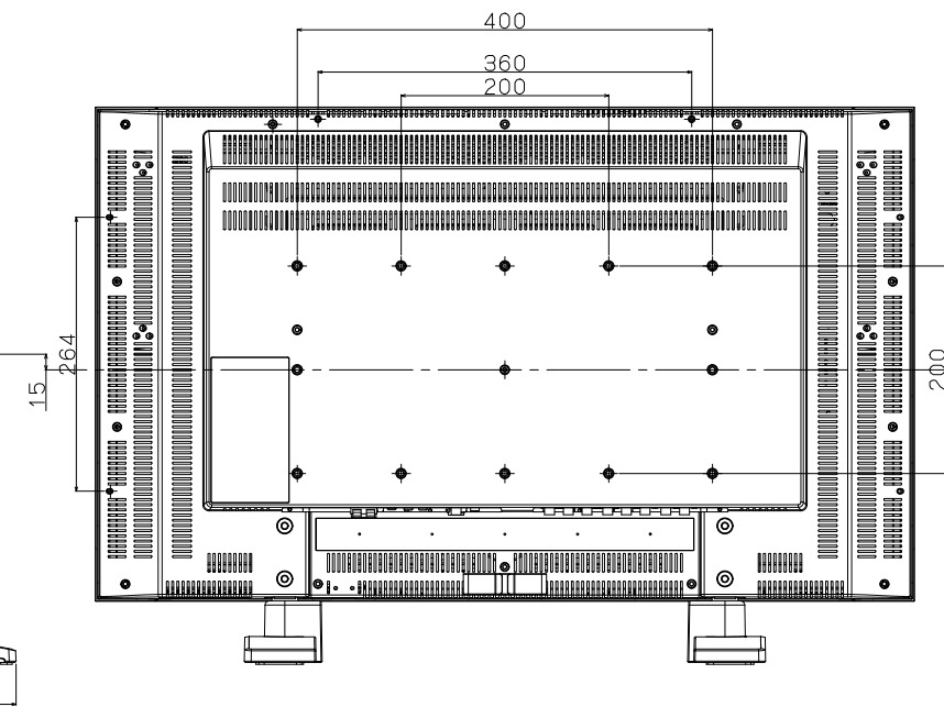
LCD3215 with ST-3215 Outside Drawing
