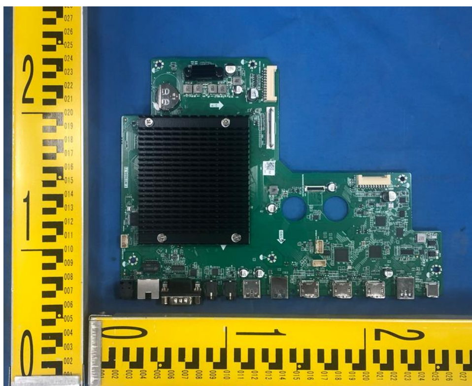
Figure 4. Mainboard view
