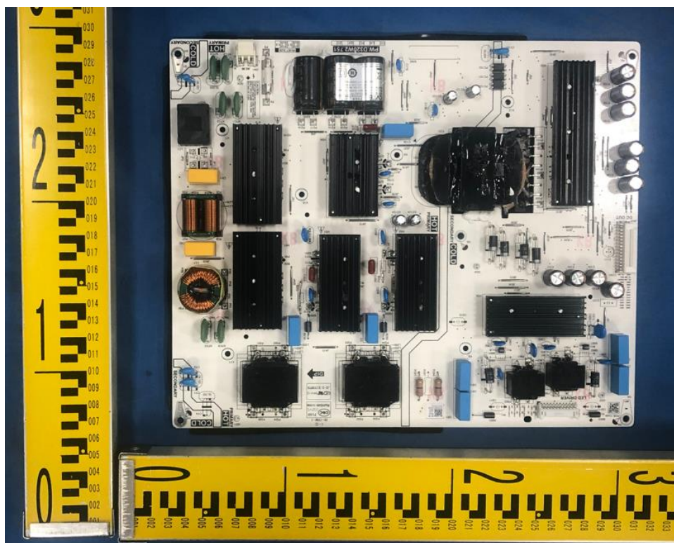
Figure 3. Power board
