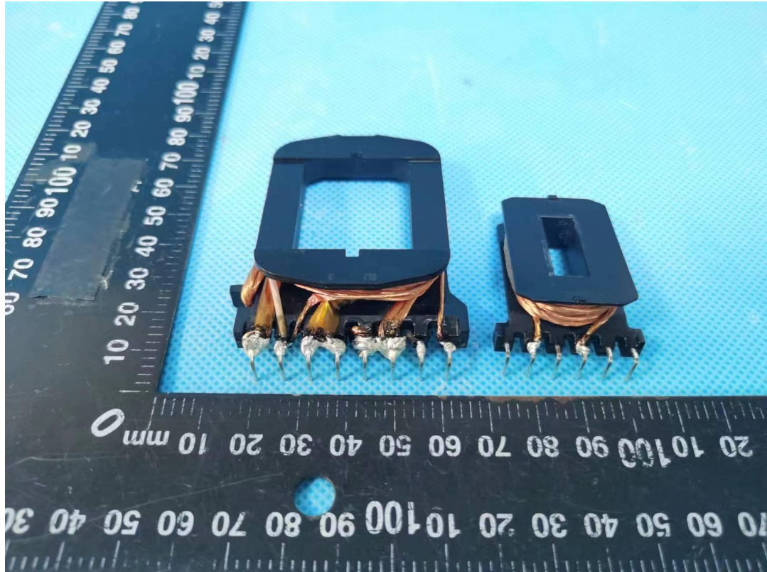
Photo 23 Transformer TH1 view
