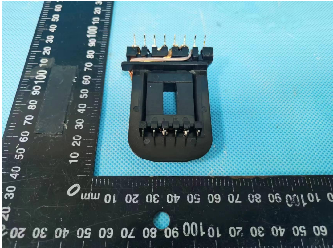
Photo 21 Transformer TH1 view
