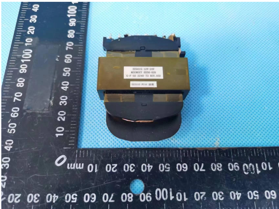
Photo 18 Transformer TH1 view
