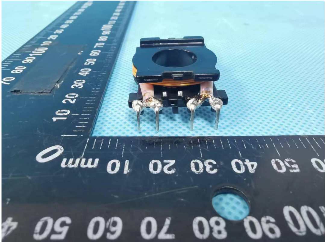
Photo 27 Transformer TF2 view
