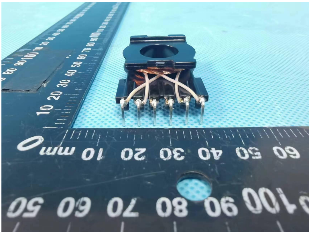
Photo 28 Transformer TF2 view
