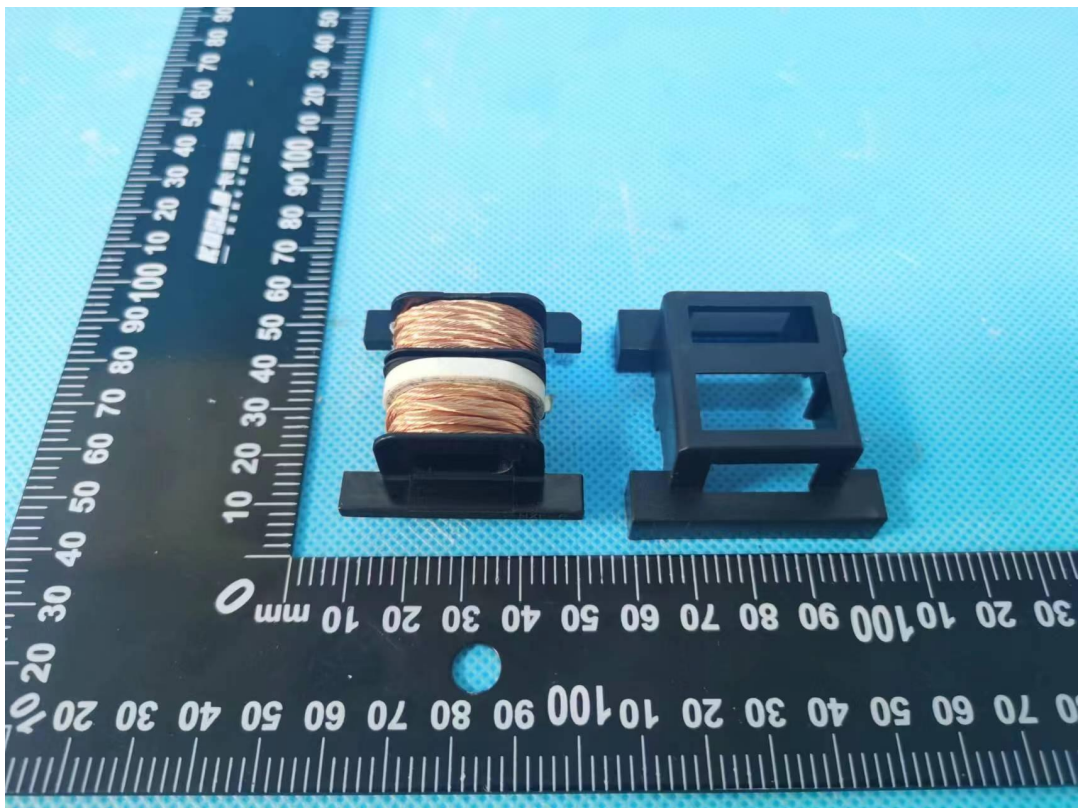
Photo 16 Transformer TH2/TH3 view
