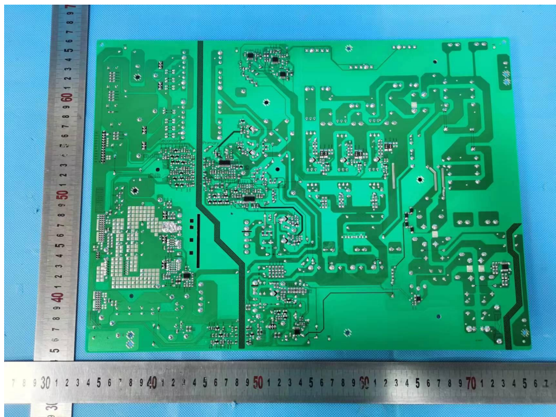
Photo 10 Power board view
