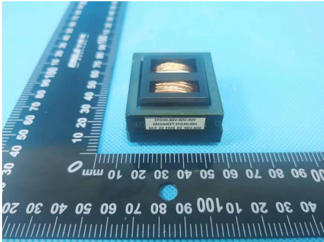
Photo 13 Transformer TH2/TH3 view
