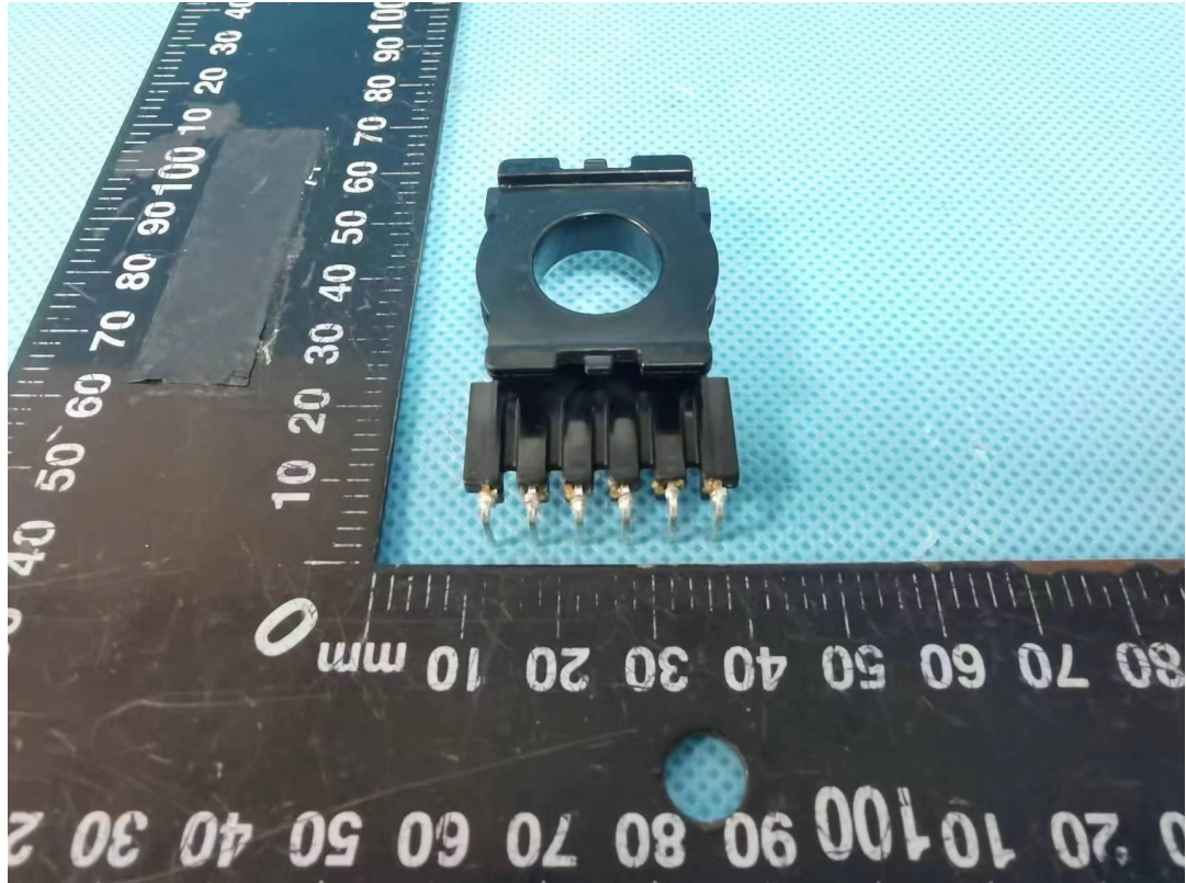
Photo 29 Transformer TF2 view
