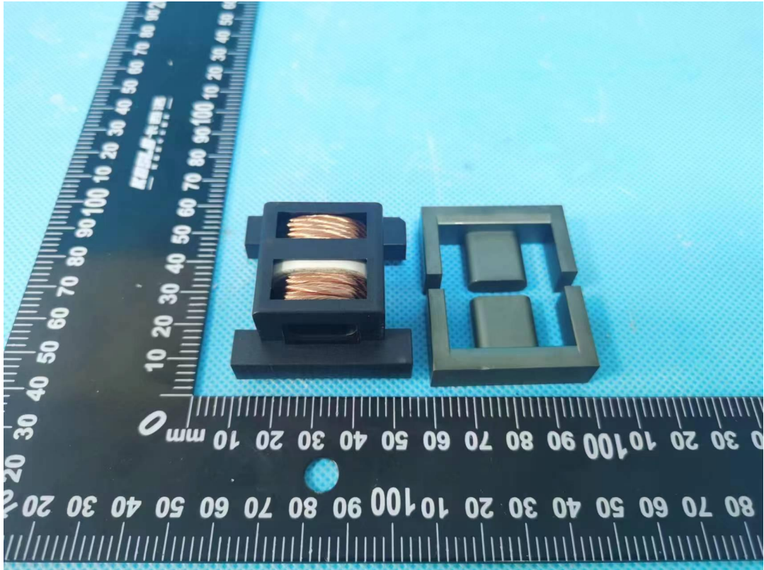
Photo 15 Transformer TH2/TH3 view
