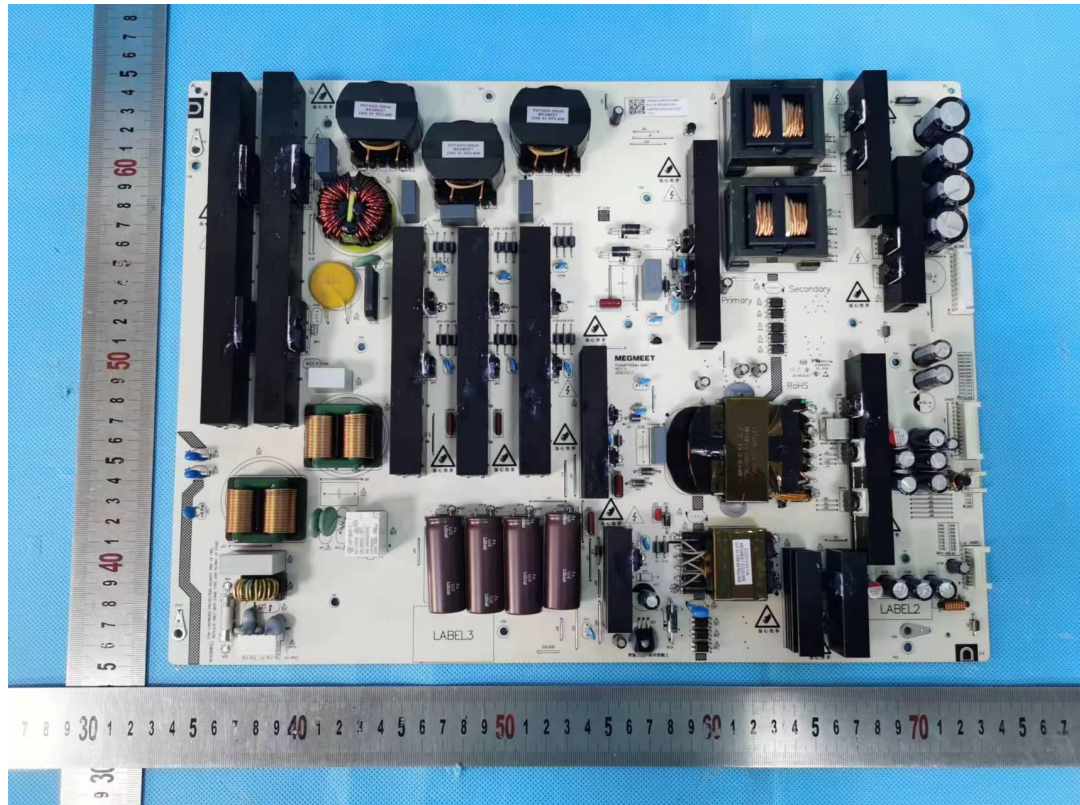
Photo 9 Power board view
