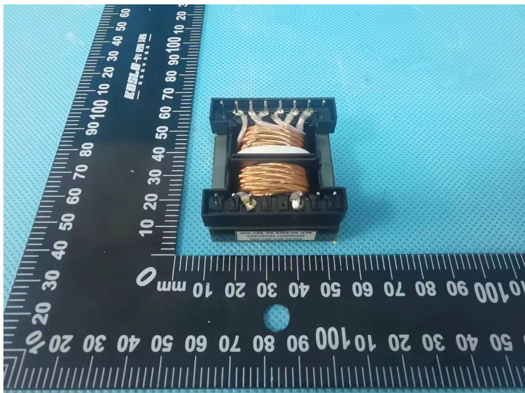
Photo 14 Transformer TH2/TH3 view
