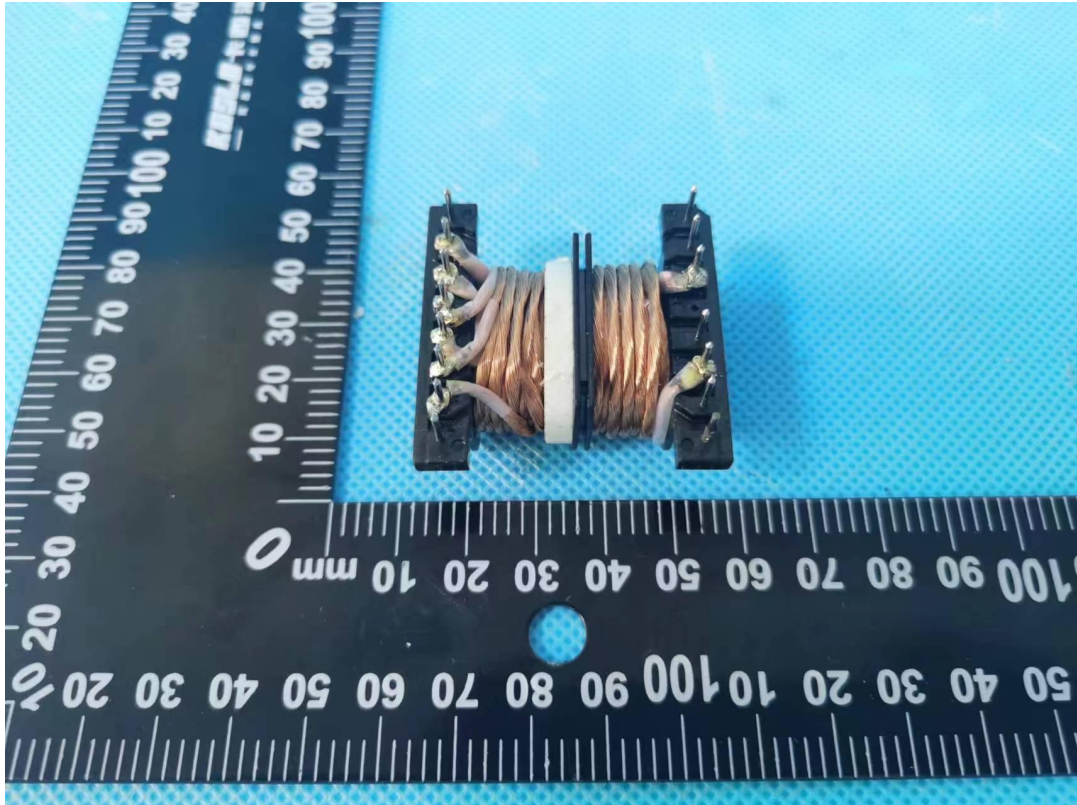
Photo 17 Transformer TH2/TH3 view
