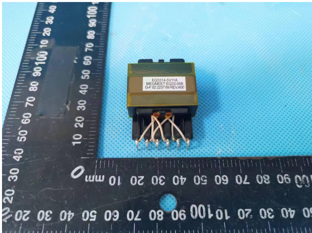
Photo 24 Transformer TF2 view
