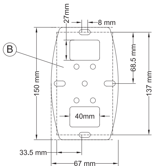
Holes pattern for ceiling plate.
