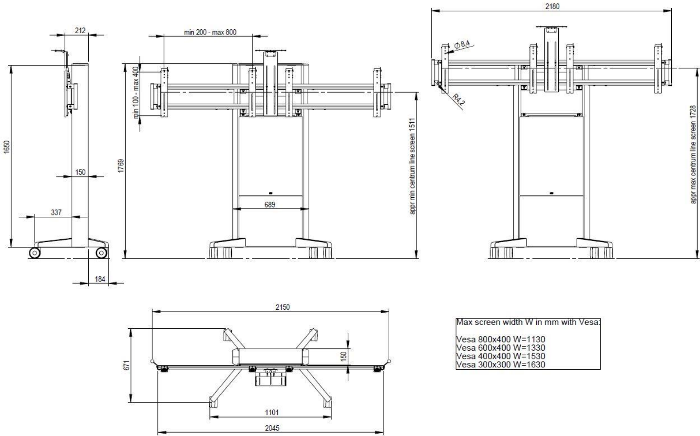
Technical drawing (mm) C5-31U0006-2-A-0 / SMS Presence Video Conference Mobile 1650
