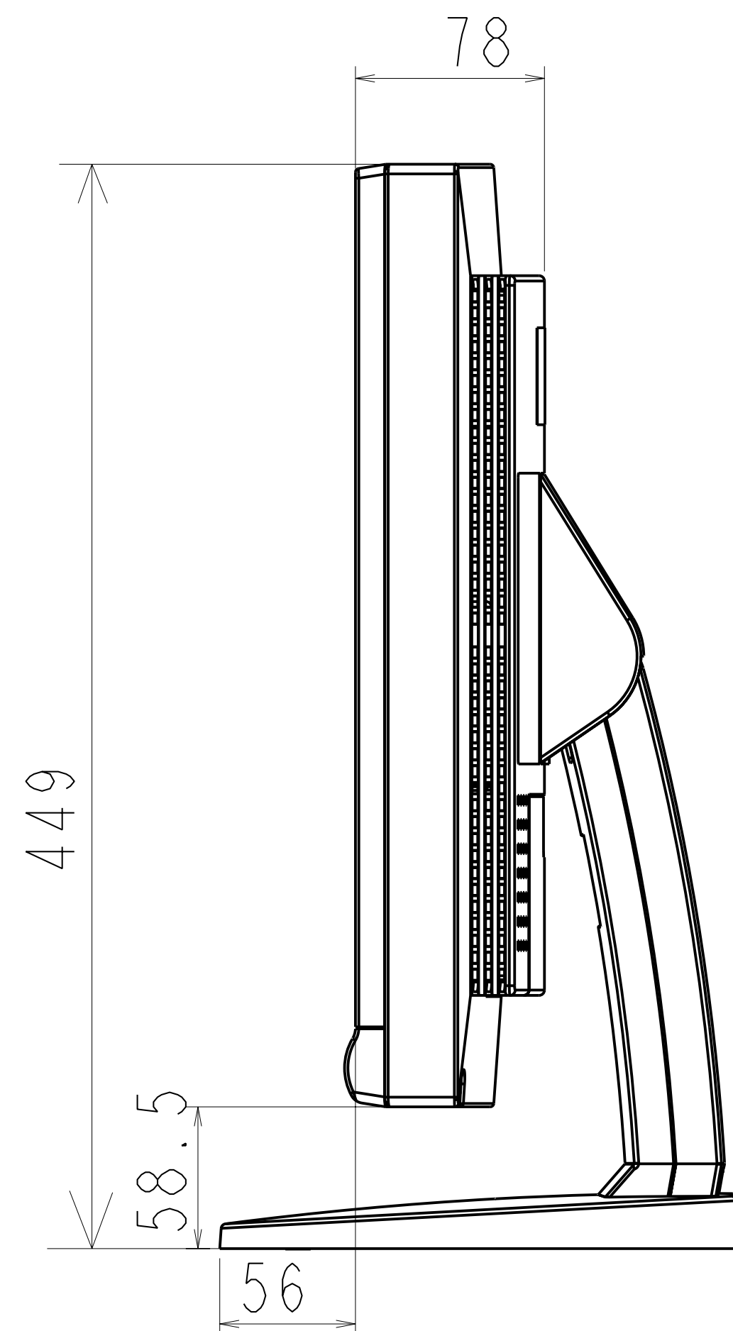
LCDI830 Outside Draw
