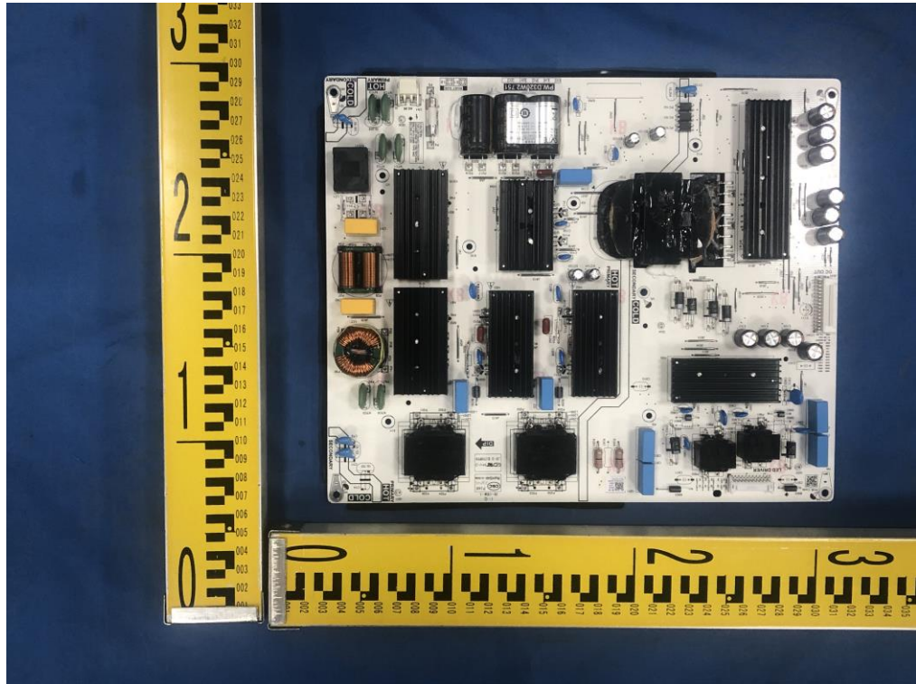
Figure 11 Switching Power Supply view
