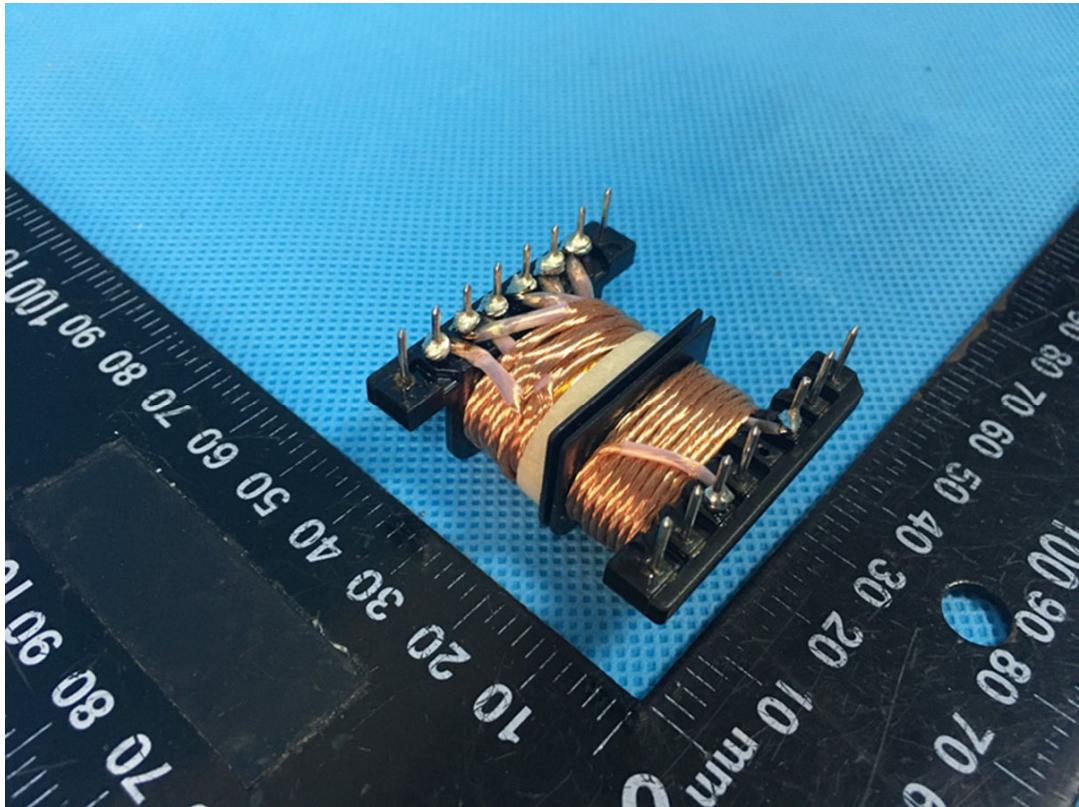
Photo 27 Transformer THA1 view
