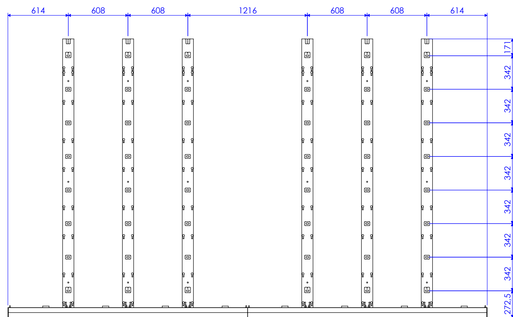
FRONT VIEW MOUNTING
