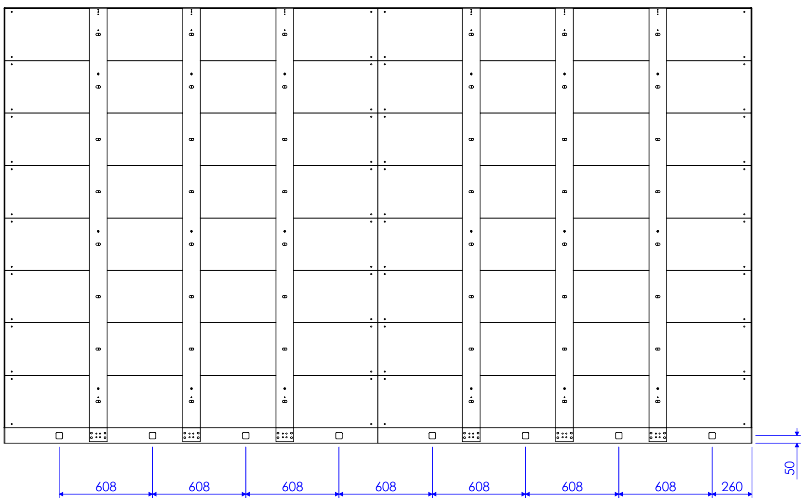
REAR VIEW CABLE HOLES
