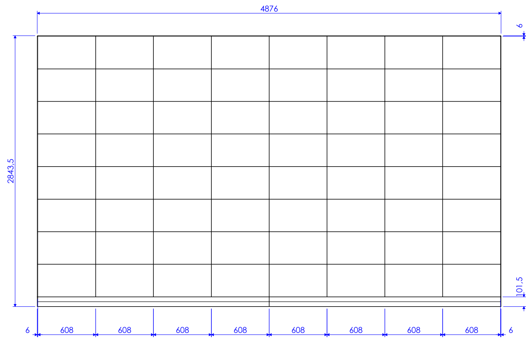
FRONT VIEW
