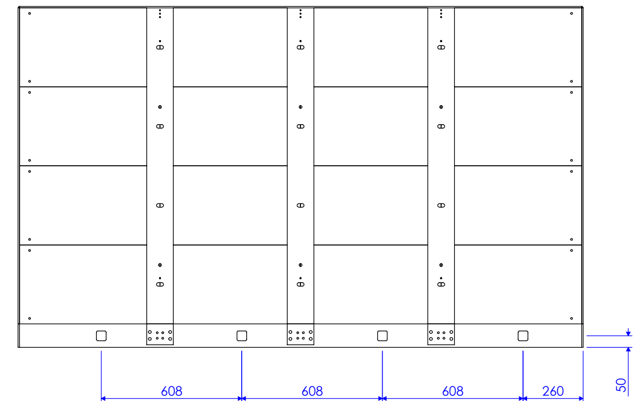
REAR VIEW CABLE HOLES
