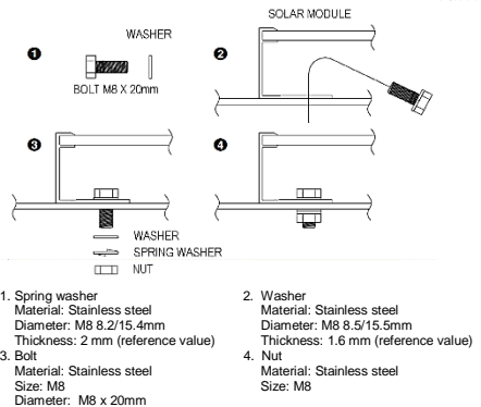
Fig. B1: The components for BOLT & NUT
