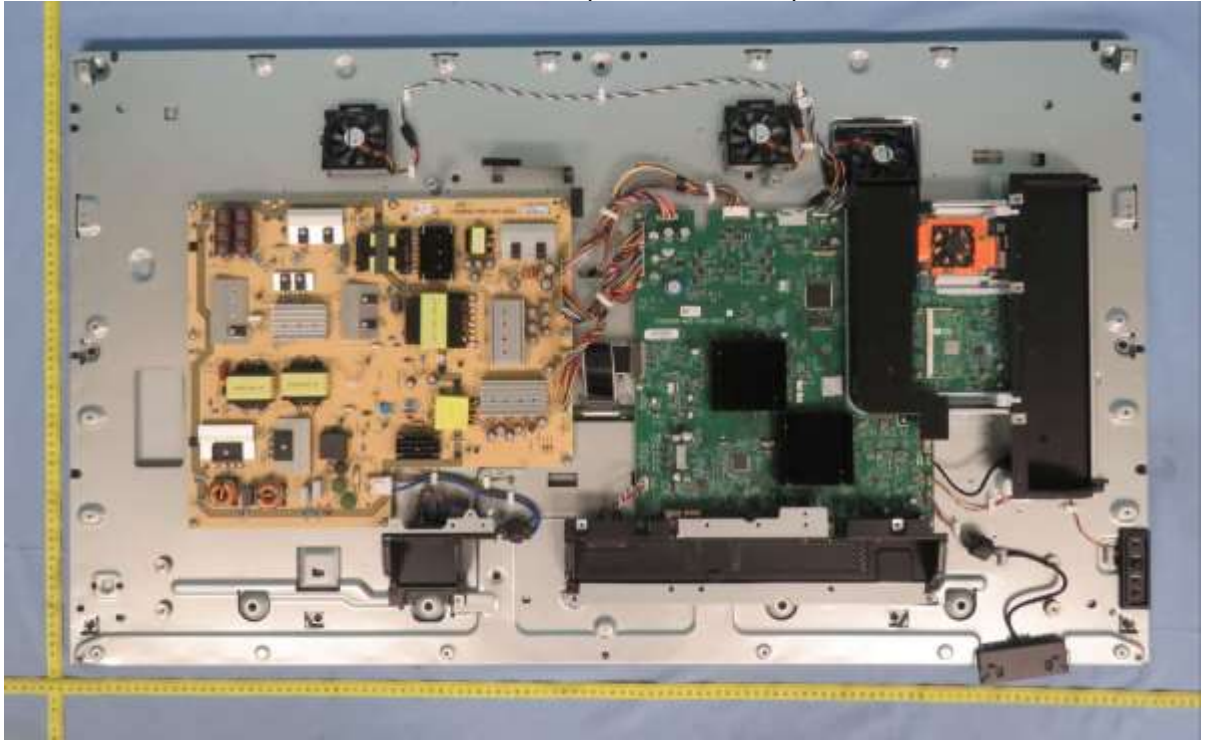
Internal view 2 (for P495, MA491)
