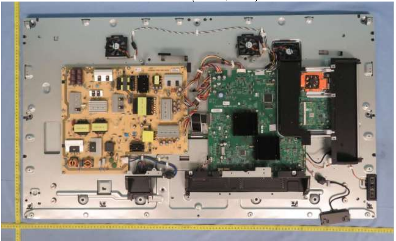
Internal view 1 (for P555, MA551)
