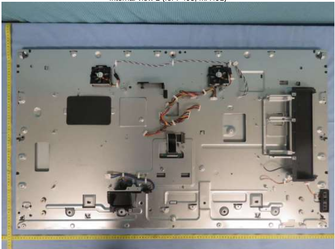
Internal view 2 (for P495, MA491)
