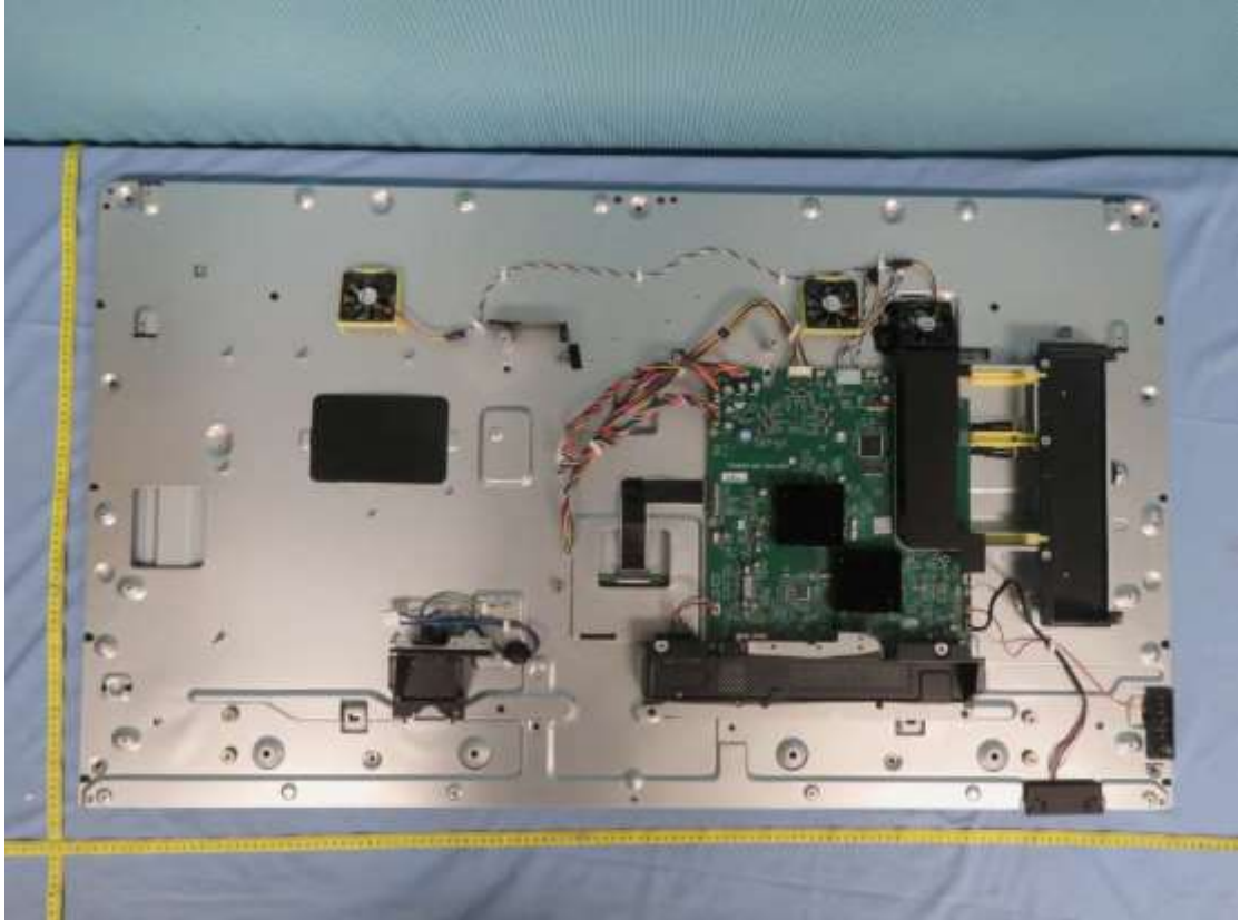
Metal enclosure internal view (for P555, MA551)
