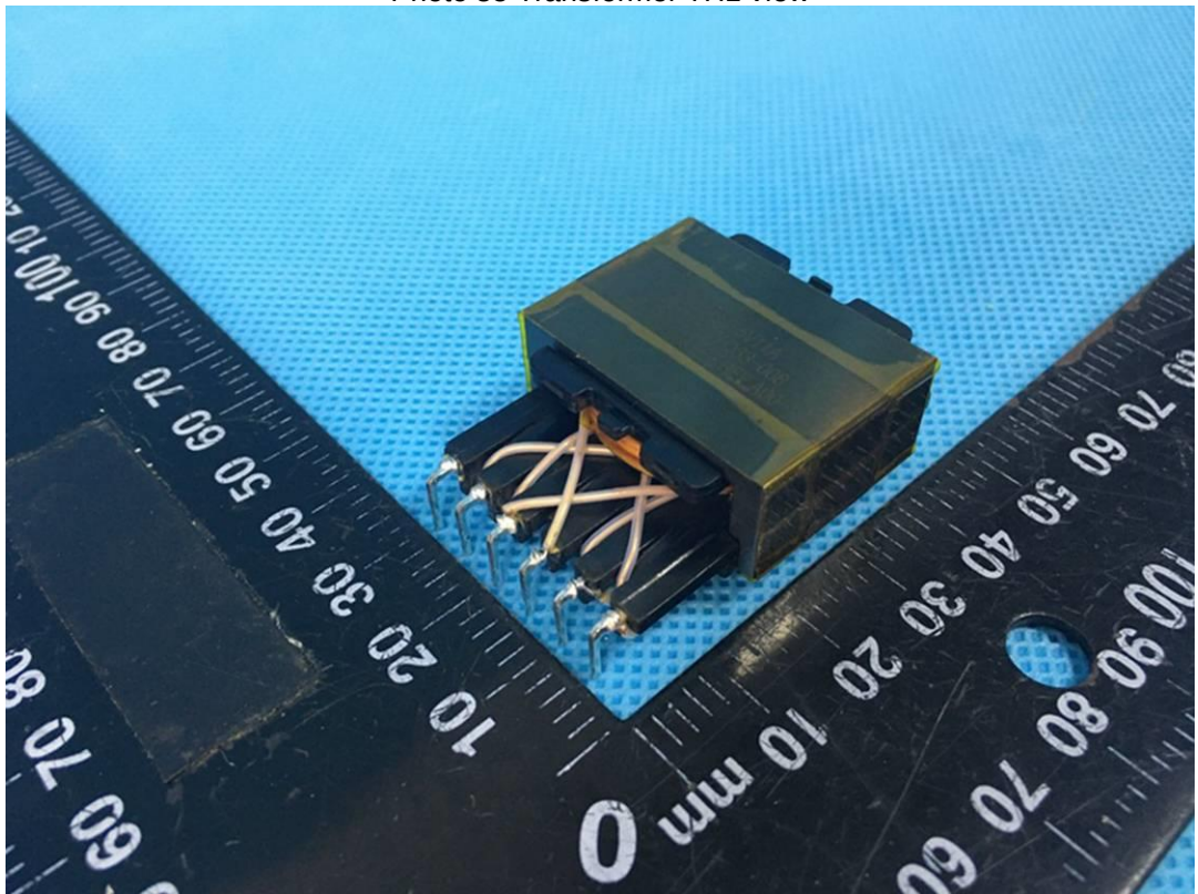
Photo 36 Transformer TF2 view
