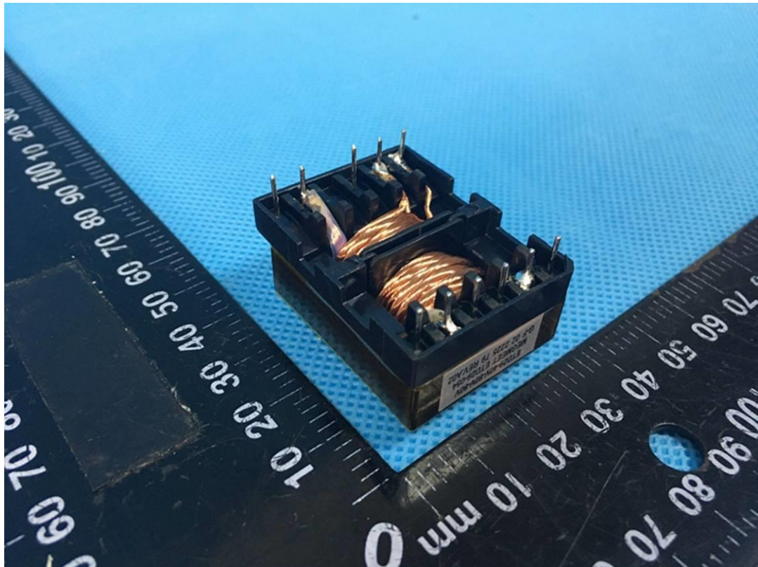
Photo 19 Transformer TH2/TH3 view
