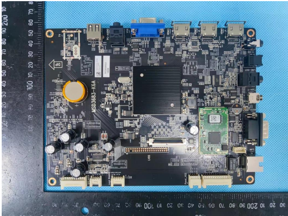
Photo 13 Main board view
