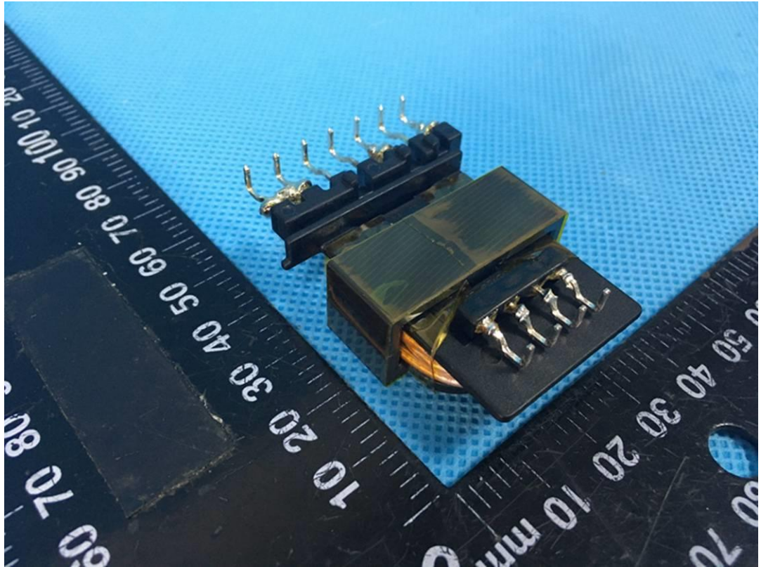
Photo 27 Transformer TH1 view
