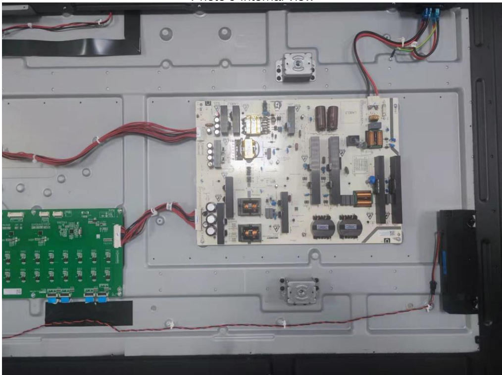
Photo 10 Internal view
