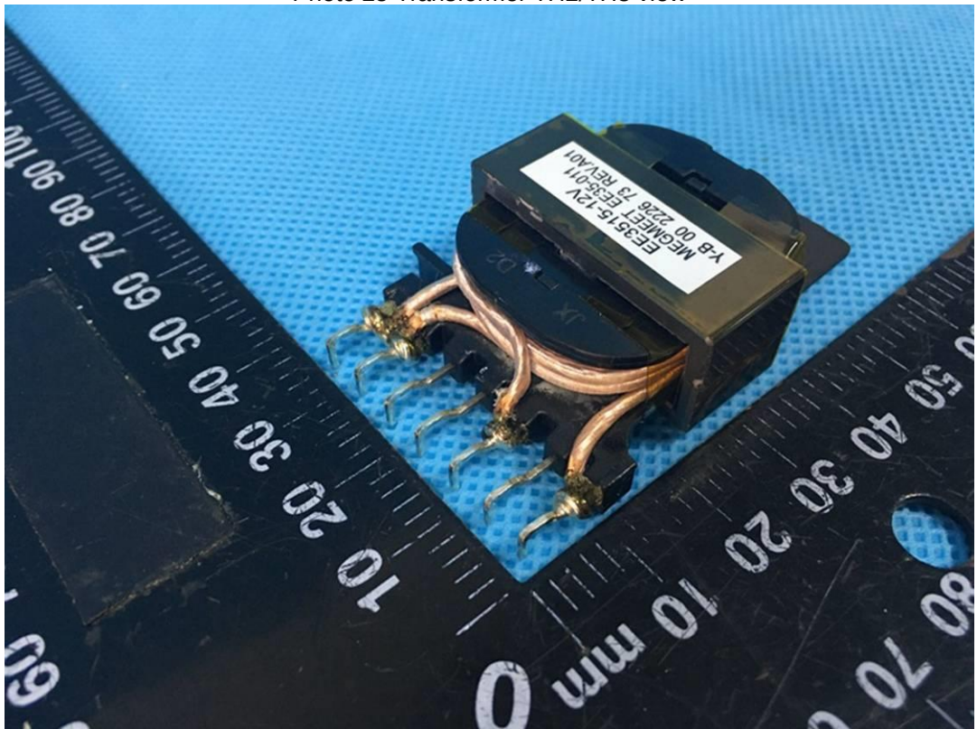
Photo 26 Transformer TH1 view
