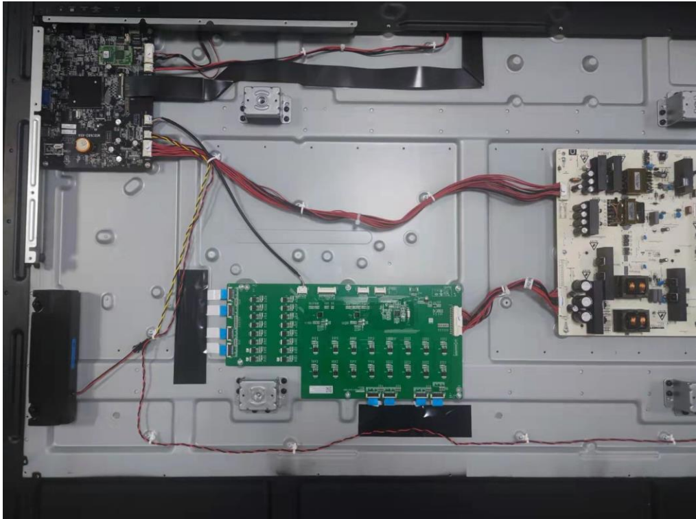
Photo 9 Internal view
