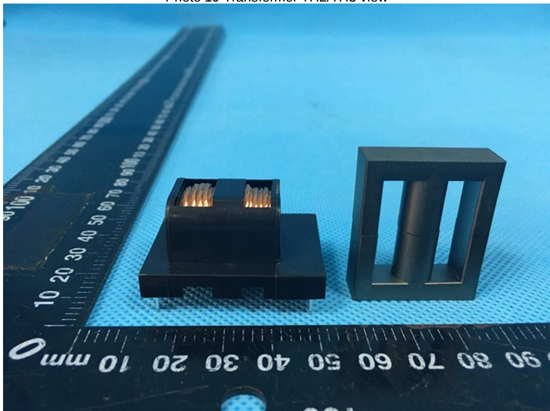
Photo 20 Transformer TH2/TH3 view
