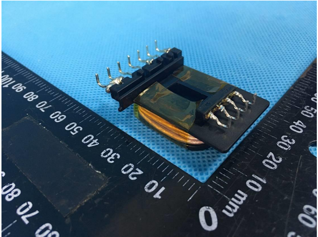
Photo 29 Transformer TH1 view
