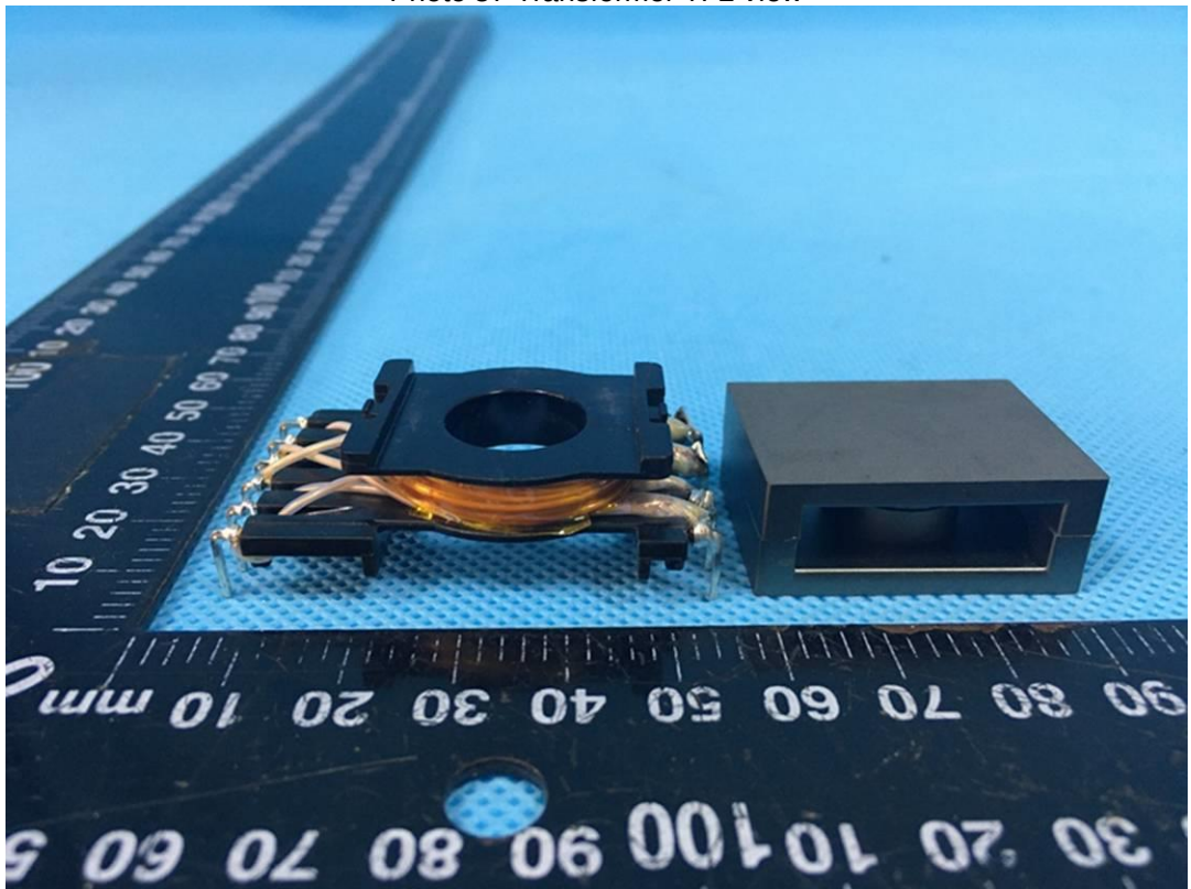
Photo 38 Transformer TF2 view
