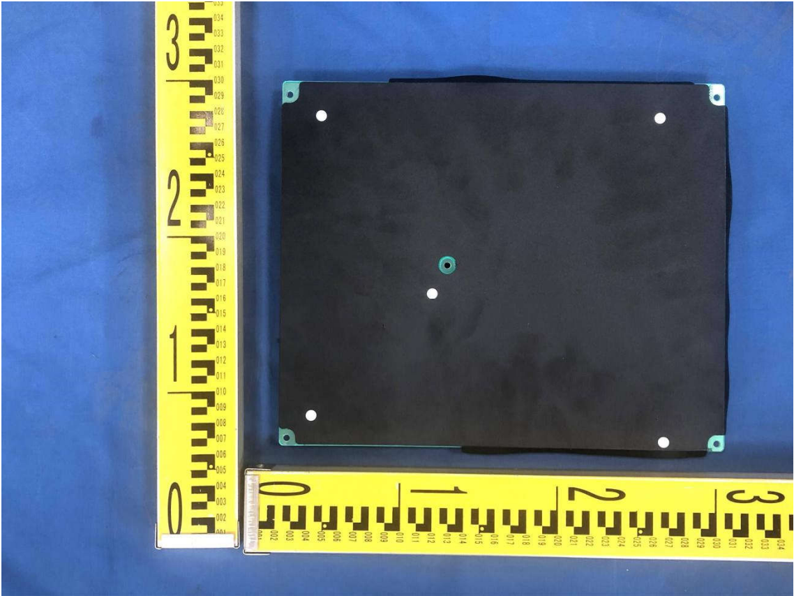
Figure 12. Power board PW.D320W2.751 Mylar sheet view
