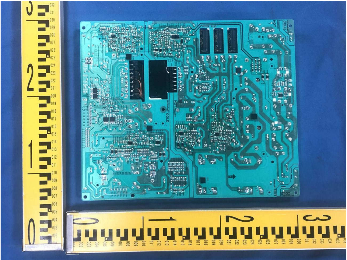
Figure 13. Power board PW.D320W2.751 solder side view
