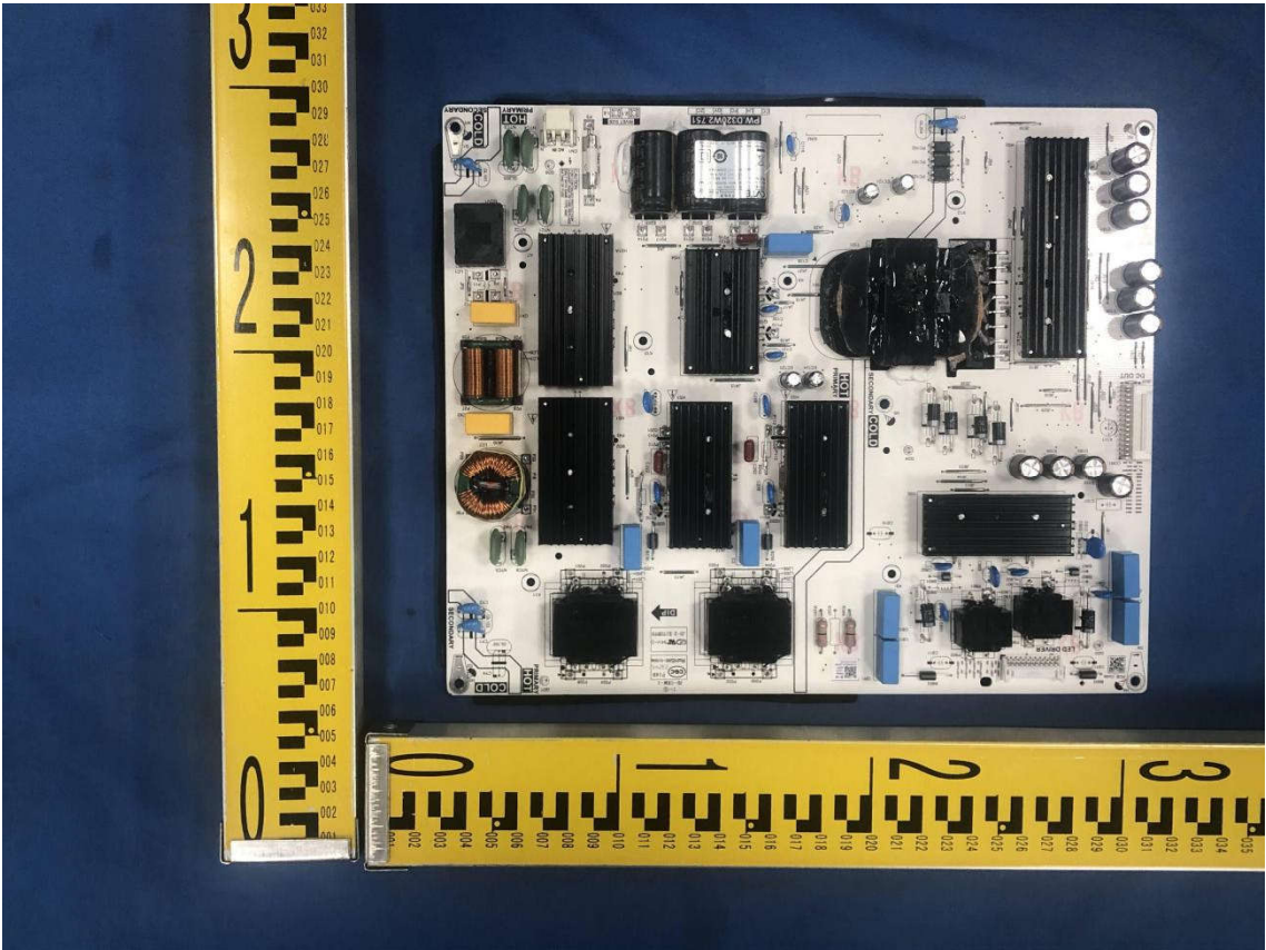
Figure 11. Power board PW.D320W2.751 component side view
