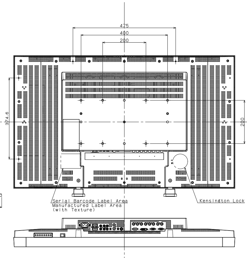
Connector Layout
