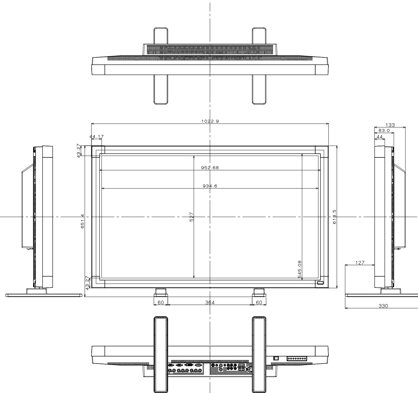
LCD4215 with ST-4020 Outside drawing
