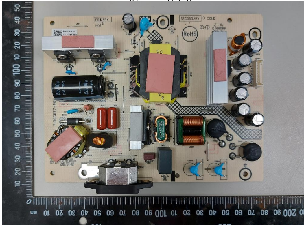
Switching power supply type A
