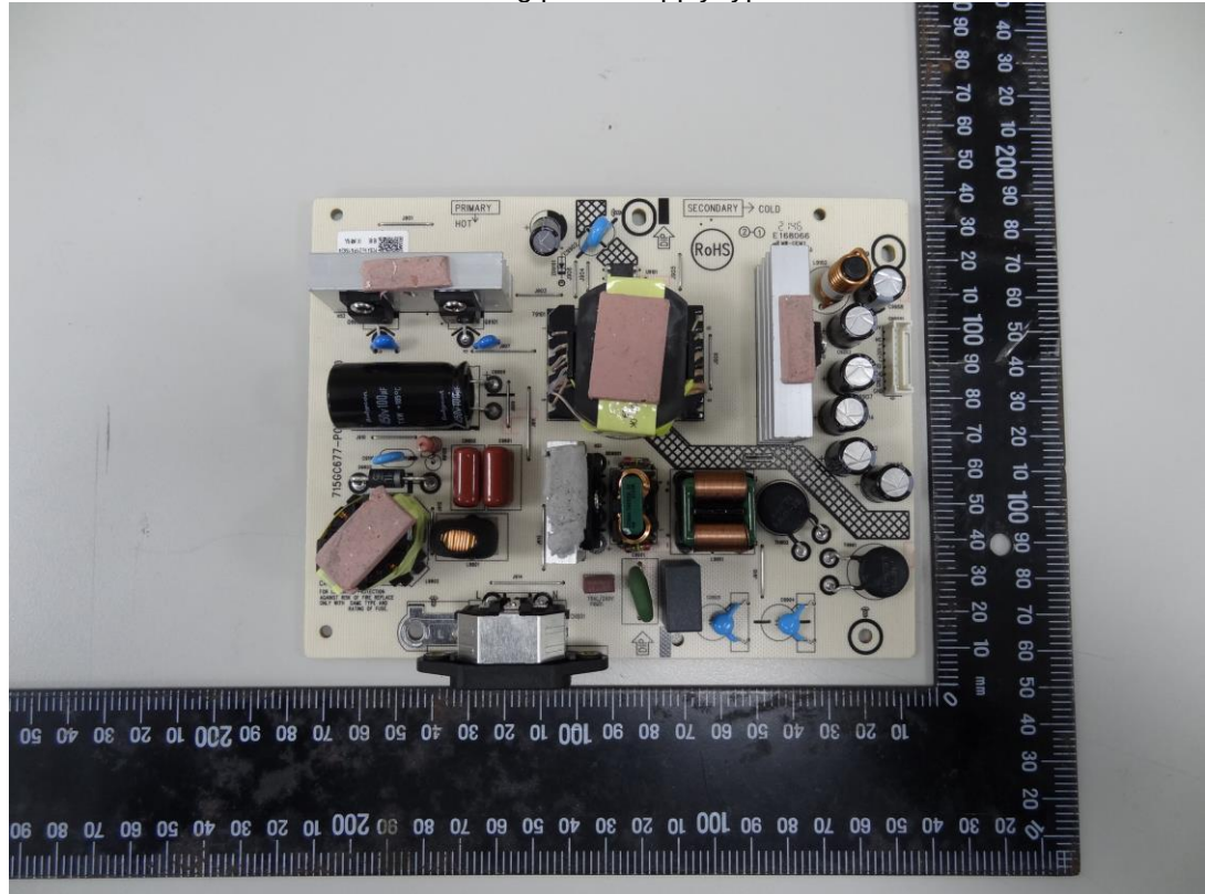
Switching power supply type B
